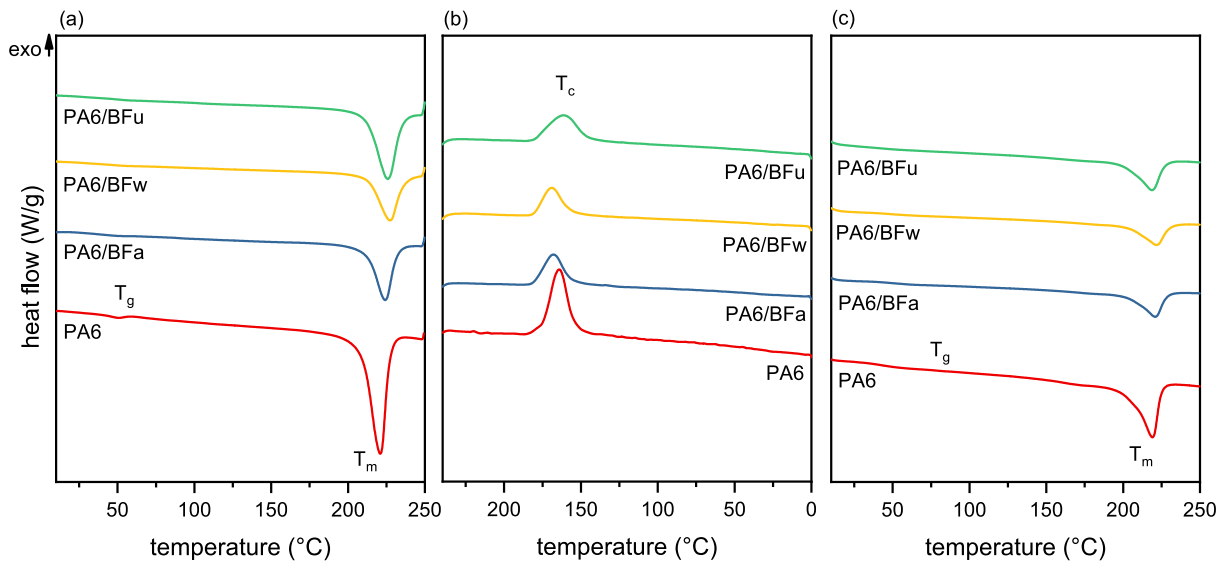
Fig. 7. DSC thermograms of the prepared composites and the neat PA6 matrix. (a) first heating scan; (b) cooling scan; (c) second heating scan.
