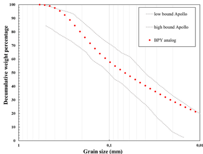
Fig. 2. Particle size distribution of the BPY analog determined by laser diffraction granulometry compared to regolith samples from Apollo missions.
