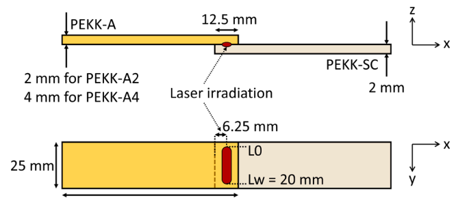
Fig. 4. Lap-joint configuration for welding PEKK-A/PEKK-SC. Schematic diagram not to scale.
