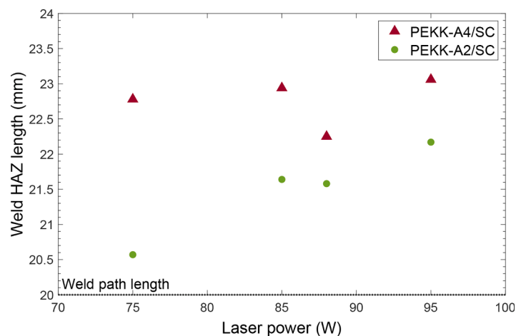
Fig. 8. Weld joint HAZ length plotted against laser power used for welding.
