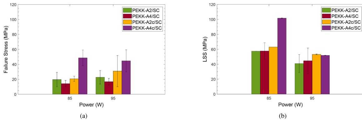
Fig. 15. Mechanical tests results of the PEKK annealed assemblies (PEKK-Ac/SC) compared with the correspondent PEKK non-annealed assemblies (PEKK-A/SC) results: (a) failure stress and (b) lap shear stress. Error bars indicate standard deviation.
