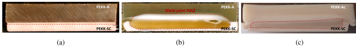
Fig. 9. PEKK-A/SC weld joint cross section a) before welding, b) after welding and c) after annealing process.
