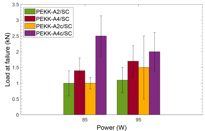
Fig. 14. Mechanical results of the PEKK annealed assemblies (PEKK-Ac/SC) showing the F_f compared with the correspondent PEKK non-annealed assemblies (PEKK-A/SC) F_f . Error bars indicate standard deviation.
