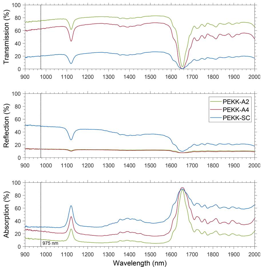
Fig. 3. Transmission, Reflection and Absorption spectra of PEKK injected plates.
