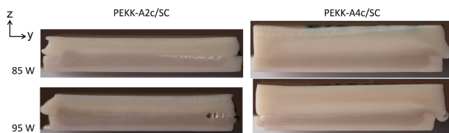
Fig. 10. Weld joints cross-section along the weld path of the crystallized assemblies (PEKK-Ac/SC).
