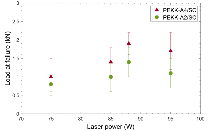
Fig. 11. Mechanical tests results showing the load at failure ( F_f ) for all PEKK-A/SC assemblies combinations. Error bars indicate standard deviation.
