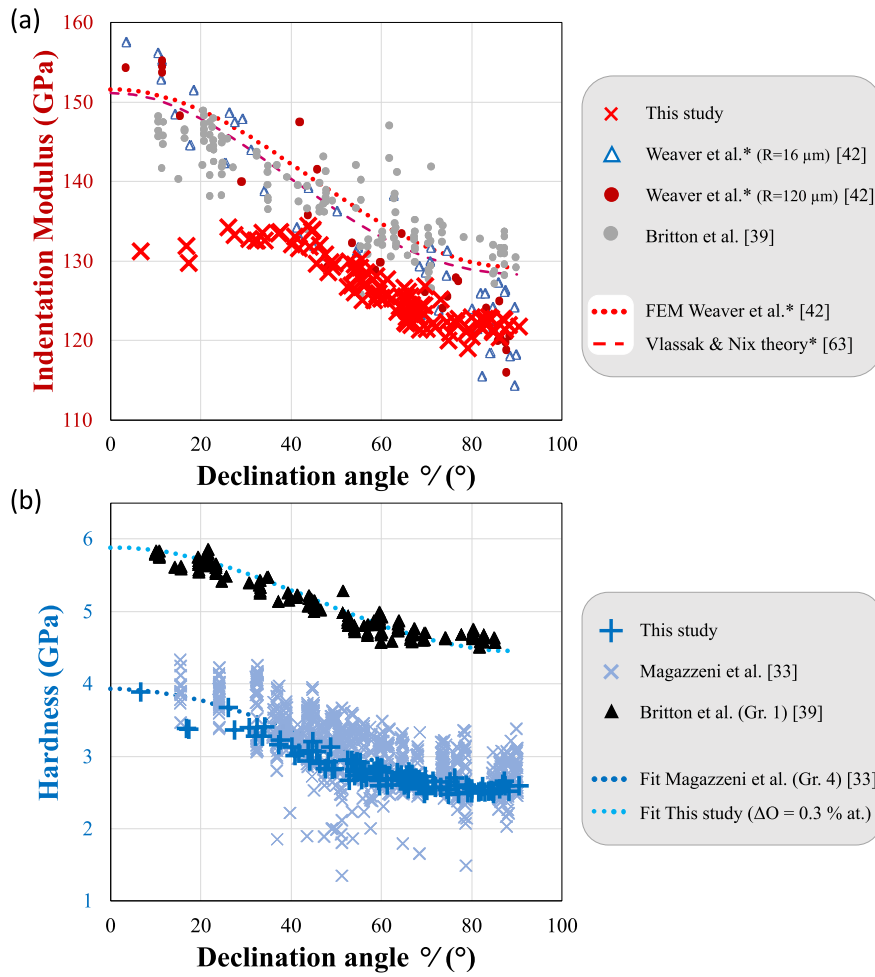
Figure 12: Evolution of the (a) indentation modulus and (b) hardness as a function of the declination angle ^\circ / compared with data and models from the literature. The asterisk corresponds to corrected values of reduced moduli considering the factor of 1.06, as was done by Aspinall et al. [75].
