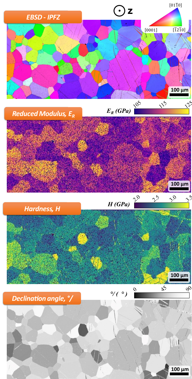
Figure 3: Grain orientation map in reference to the LTD/Z direction for the bulk CP-Ti material, Reduced modulus map using HSNM, Hardness map using HSNM, Declination ( \theta ) map computed from EBSD measurements.
