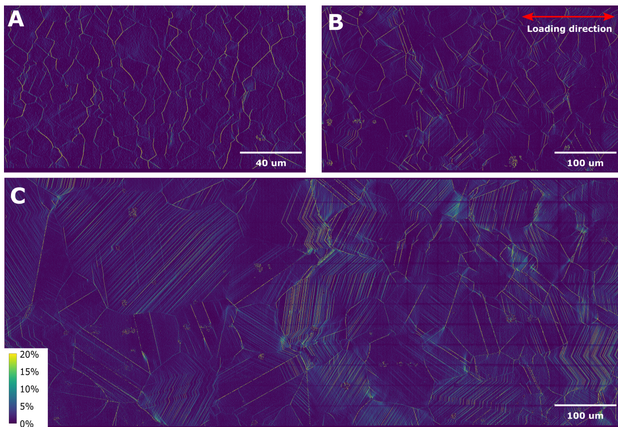
Figure 4: Strain maps obtained by HR-DIC; A. Very fine-grain microstructure; B. Fine-grain microstructure; C. Coarse-grain microstructure
