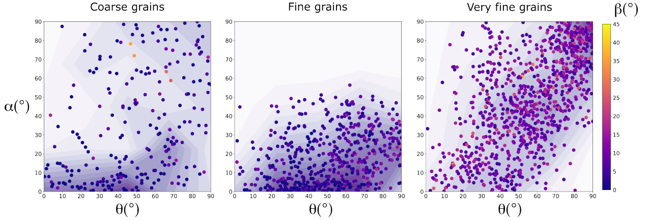
Figure 10: Grain boundary sliding characterization; Each point is a grain boundary sliding event plotted on the \alpha/\theta map. Angles are defined in the schematic illustration in Figure 9. A \theta angle of 0^\circ accounts of a GB parallel to the loading direction, and an \alpha angle of 0^\circ accounts for pure shearing. The color of the points indicates the out of plane nature of the slip event. The warmer the color, the more out-of-plane the slip is. The background is the density of the dots. The darker the color, the higher the density.
