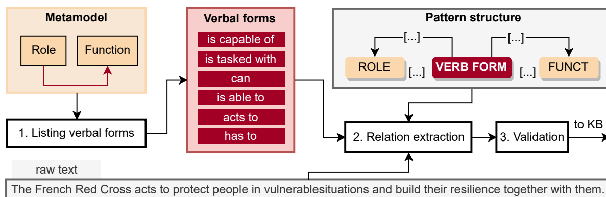
Figure 1. Proposed pattern-based extraction process of Role-Function relations
