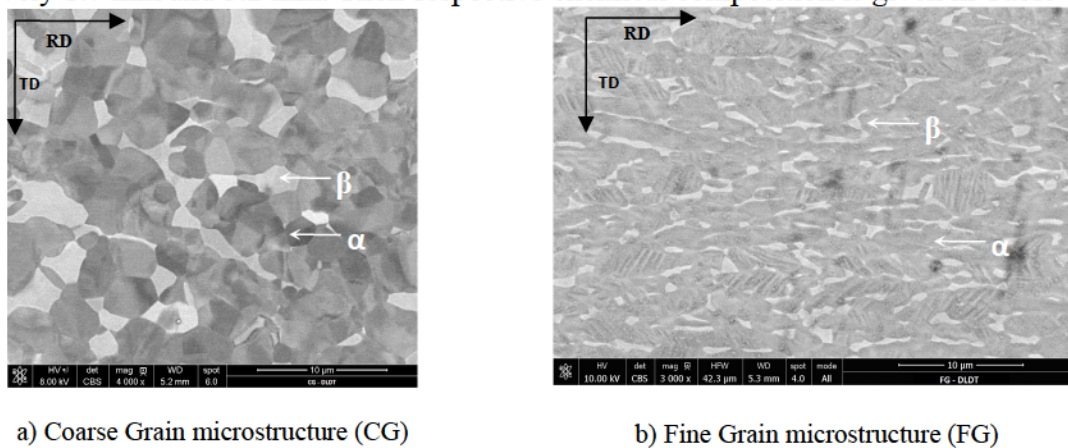
Figure 1: SEM observations of the two initial microstructures ( \alpha phase in dark and \beta phase in white)
