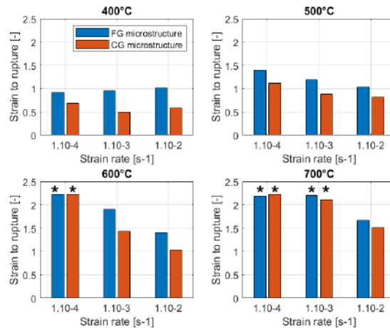
Figure 4: Strain to rupture for all temperature, strain rate and both microstructure (* last strain measured before loss of correlation)
