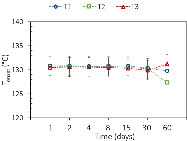
Figure 13. T_{onset} variation of sebacic acid aged with P265GH.
