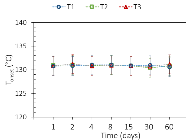
Figure 11. T_{onset} variation of sebacic acid aged with 316L.
