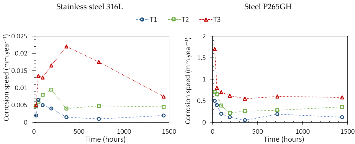
Figure 15. Corrosion kinetics of stainless steel 316L (left) and steel P265GH (right) in contact with sebacic acid at 3 different temperatures ( T_1 = 146\text{ }^{\circ}\text{C} , T_2 = 156\text{ }^{\circ}\text{C} , and T_3 = 166\text{ }^{\circ}\text{C} ).
