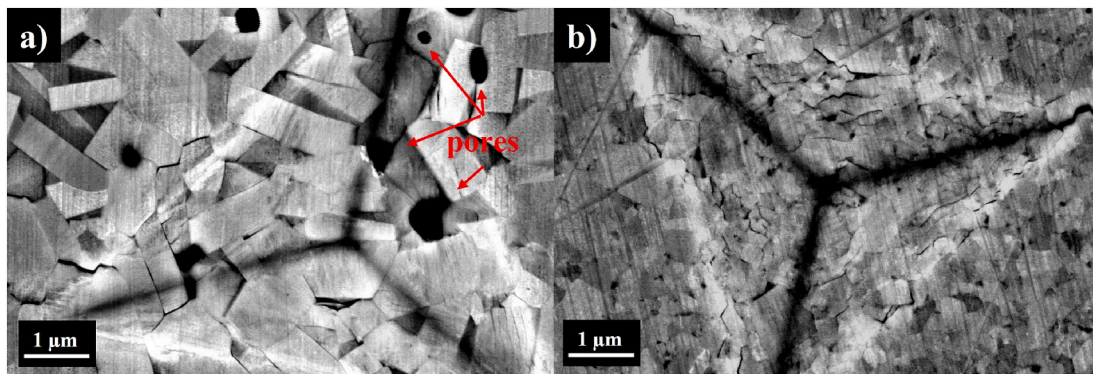
Fig. 2. Example of Berkovich imprints on FS_{\text{pure}} (a) and SPS_{\text{pure}} (b) samples at 750 mN.
