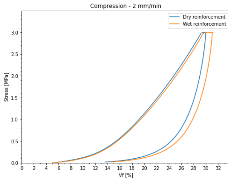
Figure 2: Stress versus V_f curve for the dry and wet CF mat preform under 3 MPa, holding force.
