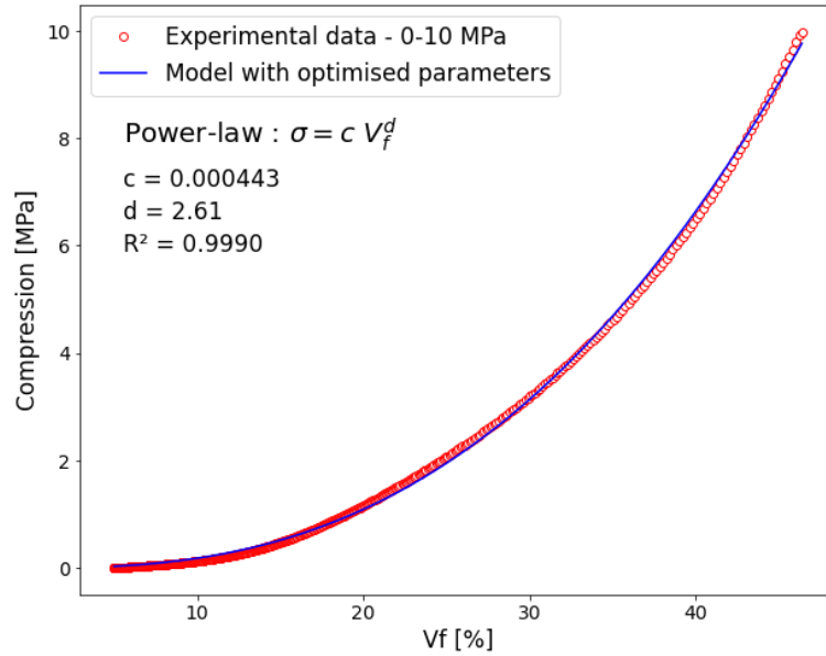
Figure 6: Modeling of the compression behavior of dry reinforcement.
