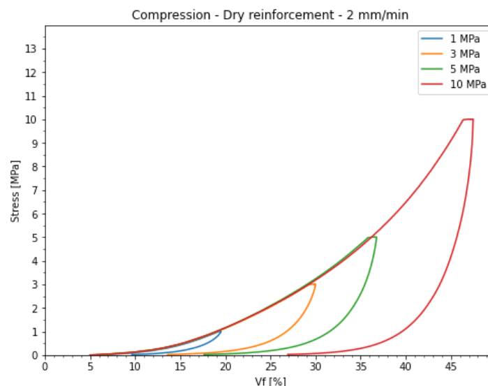
Figure 1: Stress versus V_f curves for the CF mat preform at 4 different compression levels.
