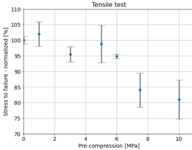
Figure 5: Effect of fiber breakage on tensile stress at break of composites.
