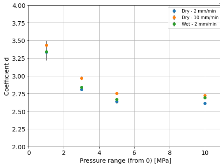
Figure 7 : Evolution of the coefficient d versus the pressure range.
