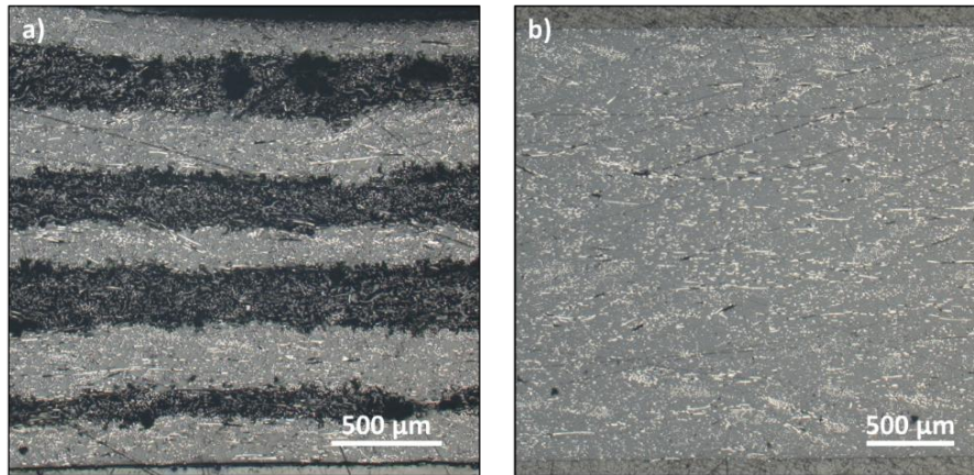
Figure 8: Optical microscope observations of composites manufactured under 1 MPa with a) M_f = 30\% et b) M_f = 20\% .
