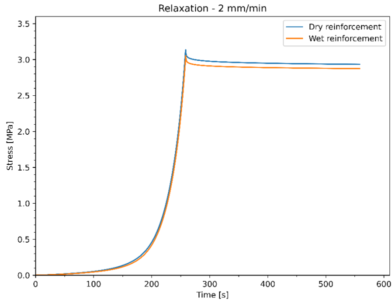
Figure 3: Evolution of the stress during the relaxation phase, holding displacement at V_f = 35\% .
