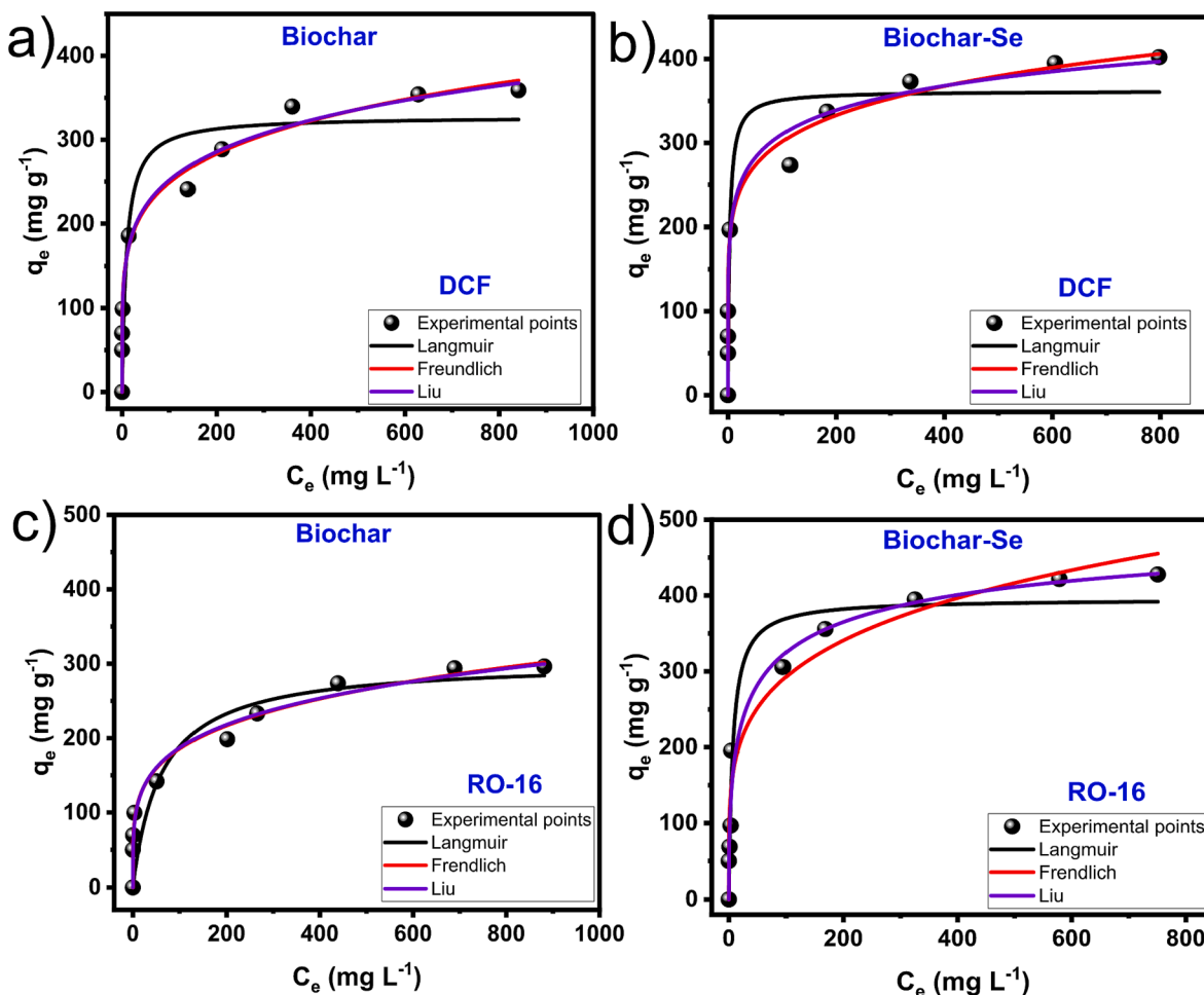
Fig. 8. Equilibrium curves at 298 K for DCF (a,b) and RO-16 (c,d) on Biochar and Biochar-Se. Conditions: initial pH 6, contact time of 40 min (DCF) and 200 min (RO-16), and adsorbent dosage of 1 g/L.
