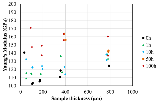
Figure 9 : Evolution of Young's modulus with oxidation duration at 700°C and sample thickness
