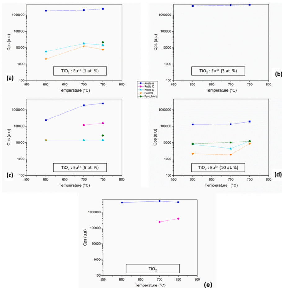
Fig. 5. Integrated peaks areas of different phases detected in Raman spectra, as a function of temperature for TiO 2 with 1 at. % (a), 3 at. % (b) 5 at. % (c), 10 at. % (d) of Eu 3+ and un-doped TiO 2 (e).
