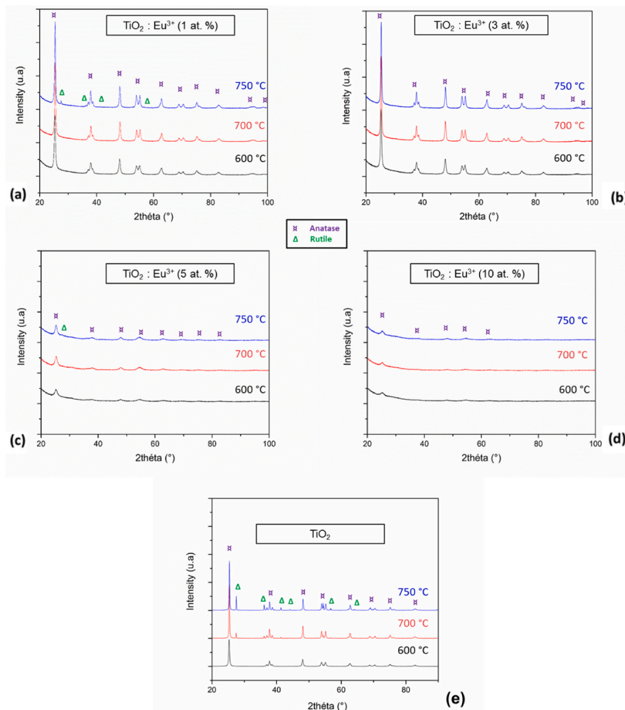
Fig. 2. XRD patterns of \text{TiO}_2:\text{Eu}^{3+} samples doped at 1 at. % (a), 3 at. % (b), 5 at. % (c), 10 at. % (d) and un-doped \text{TiO}_2 (e) heat treated at different temperatures.
