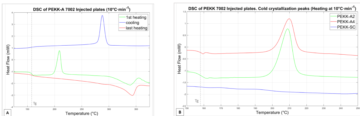
Fig. 4. (A) DSC scans of PEKK 7002 amorphous molded plates. (B) cold crystallization peaks of molded samples obtained on the first heating DSC scan.
