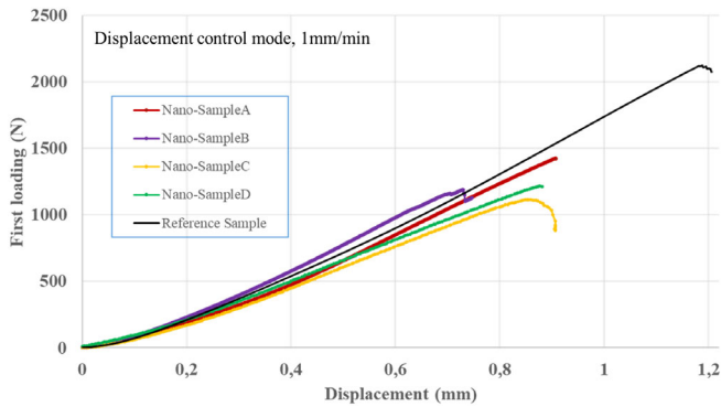
FIGURE 7 Load-displacement curves in the first loading of four nano-engineered samples and one representative reference sample.
