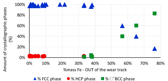
Fig. 7. Amount of crystalline phases (XRD Analyses) versus the surface mass iron content (EDS-SEM) identified at the surface of the coatings before tribological tests.
