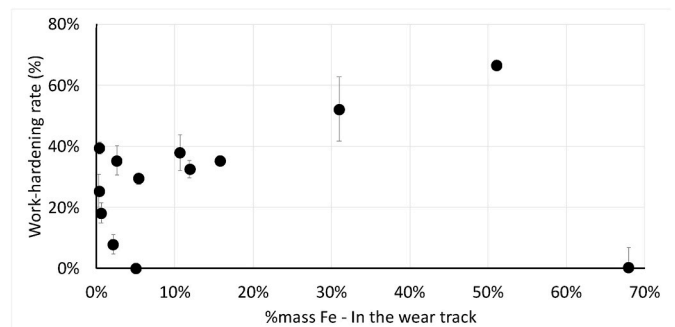
Fig. 18. Evolution of the work-hardening versus the iron content at the surface of the cobalt-based alloy after tribological tests.
