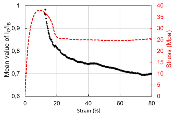
Fig. 8. Stress/strain curves and means value of I_G/I_B ration in the stretched area for 1 wt% PP/BBS film.
