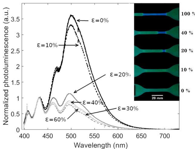
Fig. 4. Photoluminescence spectra (normalized at 430 nm) of the specimen in the stretched area for several strains and color images of the stretched specimen (1 wt% PP/BBS film).
