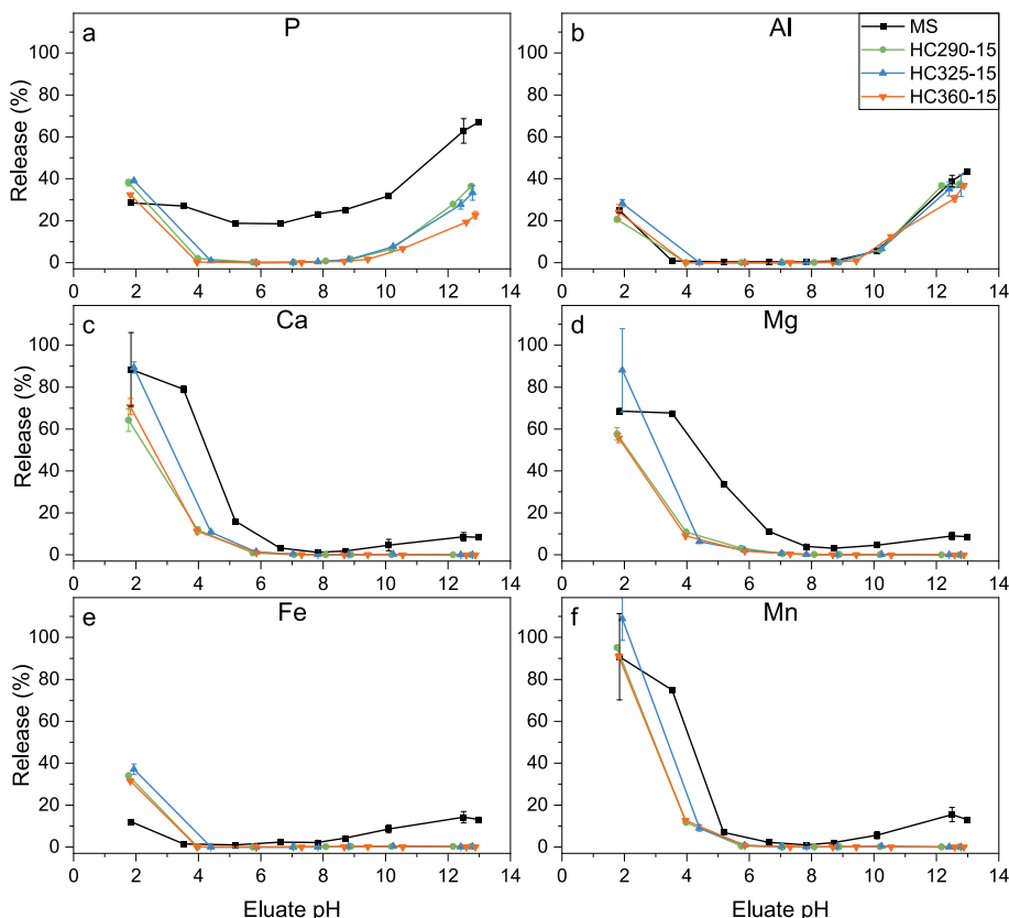
Fig. 8. Release of P and major metals from MS and hydrochar as a function of pH. Extraction conditions: L/S = 10 mL/g-dry, 30 rpm, 22 \pm 1 °C, and 24 h.
