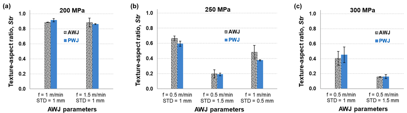
Fig. 17. Surface texture after AWJ milling and PWJ cleaning for different AWJ process parameters, (a) P = 200 MPa, (b) P = 250 MPa and (c) P = 300 MPa.
