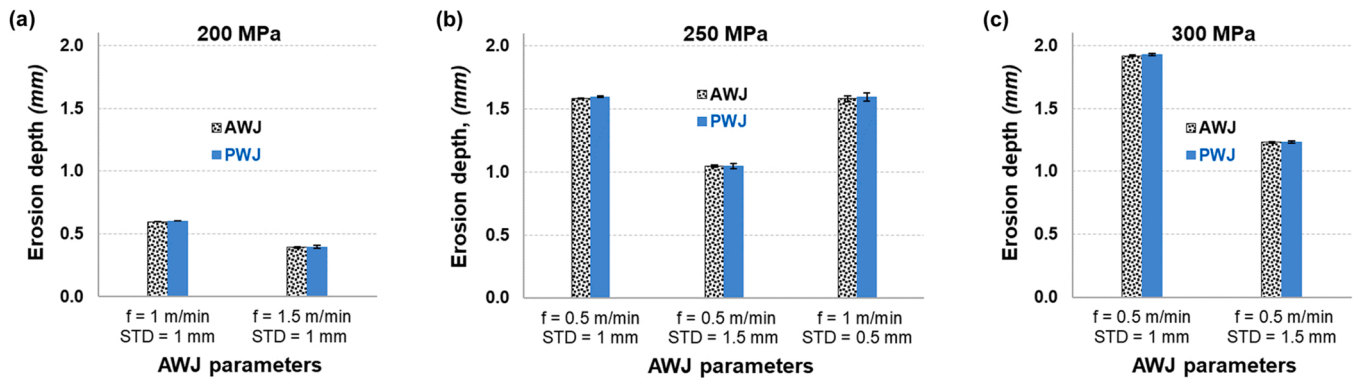
Fig. 22. Material erosion thickness after AWJ milling [20] followed by PWJ cleaning for specimens milled at different process parameters, (a) P = 200 MPa, (b) P = 250 MPa, (c) P = 300 MPa. (The thickness of bulk plate material was 3.71 mm before AWJ milling).
