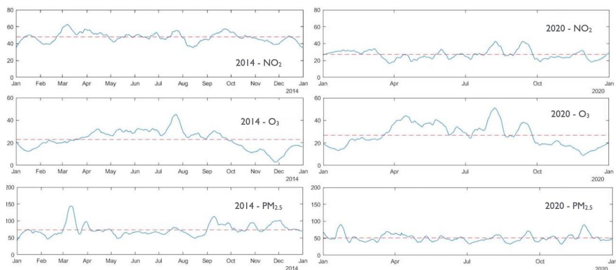
Figure 2. Annual evolution of the three air quality indicators in 2014 and 2020.
