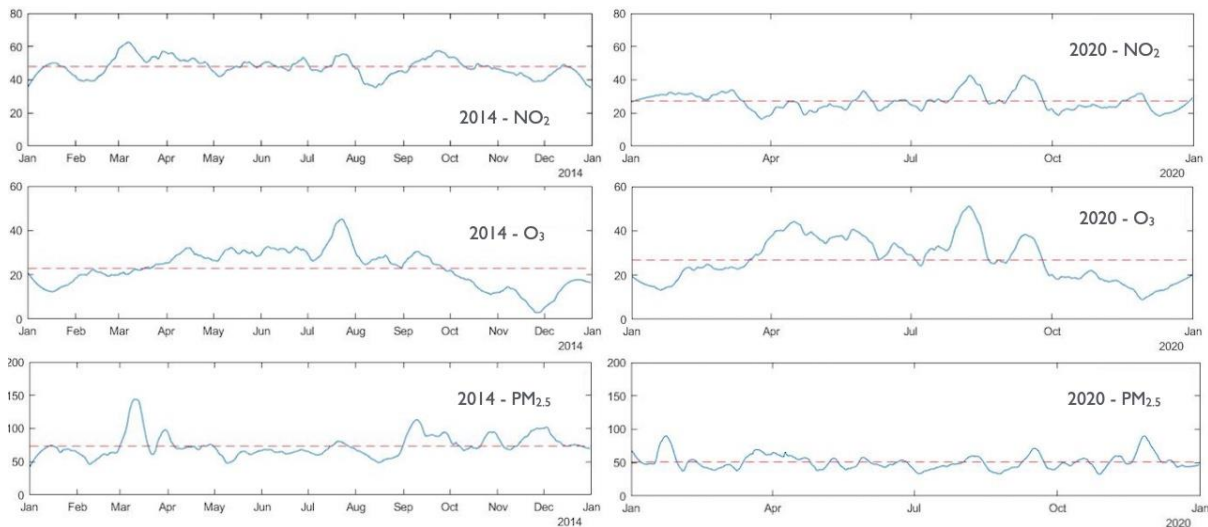
Figure 2. Annual evolution of the three air quality indicators in 2014 and 2020.
