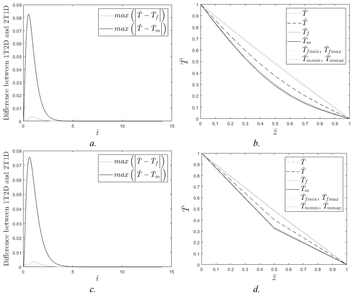
Fig. 5. 1T2D and 2D1T results for \bar{Z} = 1 , Bi_f = 5 \cdot 10^{-2} , \frac{k_r}{k_z} = 1 and \frac{k_m}{k_z} = 0.2 ; (a. and c.) maximum gap between average temperature; (b. and d.) temperature fields along \bar{z} -axis when the gap is maximum with (a. and b.) 11 and (c. and d.) 3 nodes
