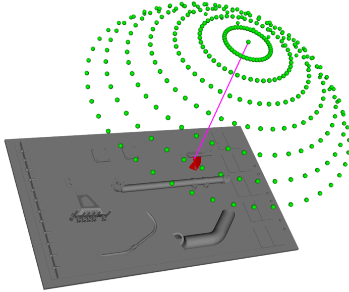
Fig. 7 Example of visibility sphere to sample camera viewpoints during rendering. Green dots are sampled camera locations, and the red object is the target object to be rendered. While rendering, the CAD of the target object is loaded and the context (here in gray) is not loaded for rendering.
