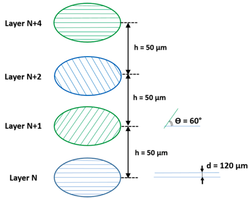
Fig. 1. SLM manufacturing strategy (example of 4 layers).
