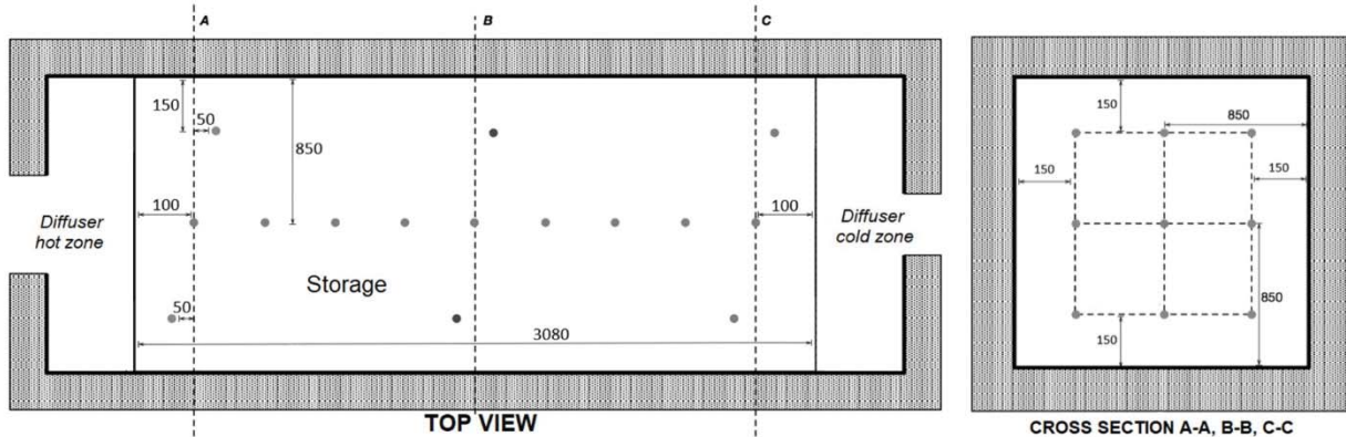
FIGURE 3. Instrumentation
