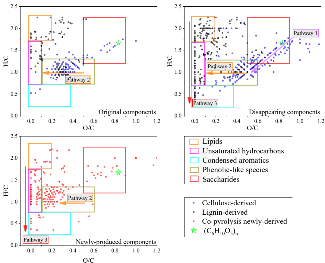
Fig. 6. Bio-oil heavy components of different origins in the van Krevelen diagrams, with original components and disappearing components sub-divided into cellulose-derived and lignin-derived components, respectively.
