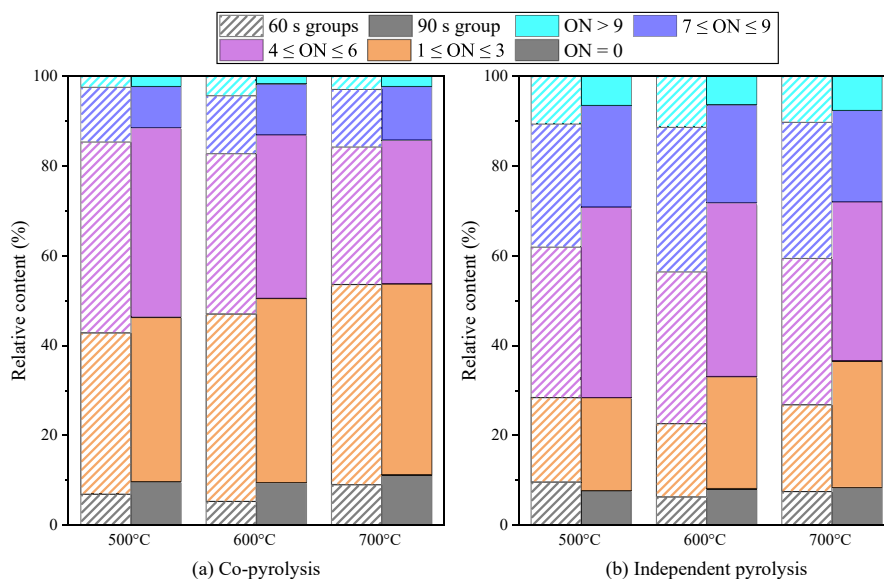
Fig. 5. Percentages of different O-containing species in heavy compounds in (a) co-pyrolysis oil and (b) independent pyrolysis results at 500, 600 and 700 °C for 60 s and 90 s.
