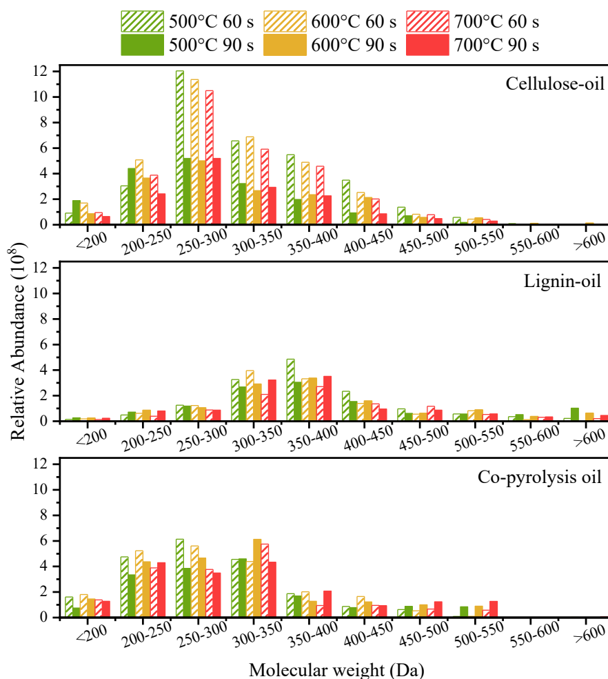
Fig. 3. Mass distributions of heavy components from the cellulose-oil, lignin-oil and co-pyrolysis oil.
