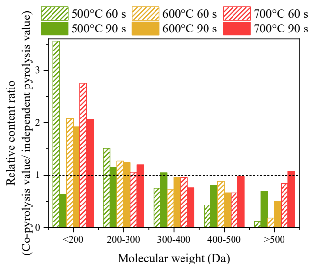
Fig. 4. Effects of cellulose-lignin interaction on mass distributions, marked by relative content ratio (co-pyrolysis value/ independent pyrolysis value).
