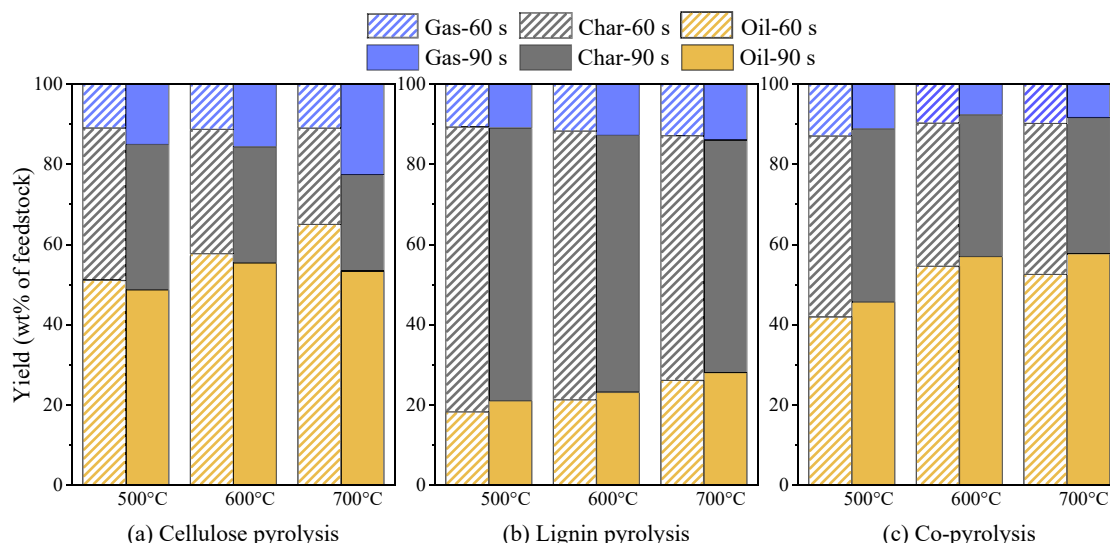
Fig. 2. Yields of bio-oil, char and gas from cellulose pyrolysis, lignin pyrolysis and co-pyrolysis (bio-oil yields are calculated by difference).
