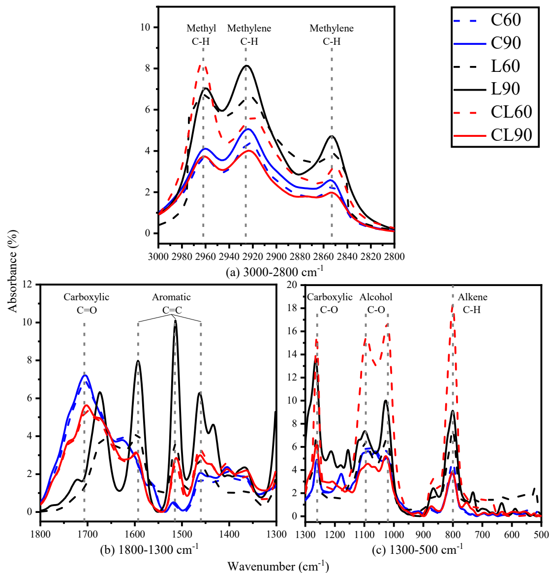
Fig. 8. FTIR absorbance spectra of bio-oil samples produced at 600 °C for 60 s and 90 s. Wavenumber scales: (a) 3000–2800 \text{cm}^{-1} , (b) 1800–1300 \text{cm}^{-1} , (c) 1300–500 \text{cm}^{-1} . C, L and CL represent cellulose-oil, lignin-oil and co-pyrolysis oil, respectively.
