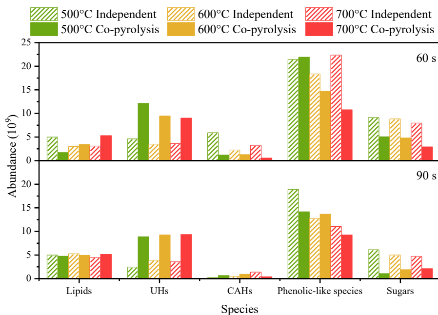
Fig. 7. Abundances of different species derived from independent pyrolysis and co-pyrolysis of different reaction time and temperature (UHs: unsaturated hydrocarbons; CAHs: condensed aromatic hydrocarbons).
