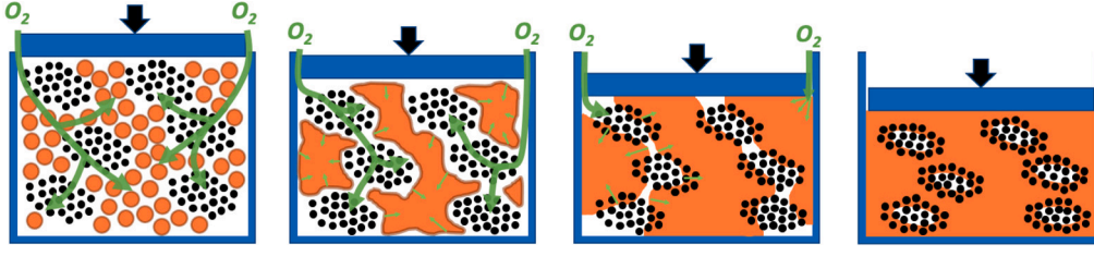
Fig. 12. Schematic representation of oxygen transport within a composite preform during compression molding processing.
