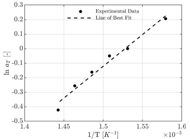
Fig. 4. Arrhenius plot of raw PEEK initial viscosity at t = 0 . The activation energy of initial viscosity E_a is obtained from the slope of the linear regression according to Eq. (2).
