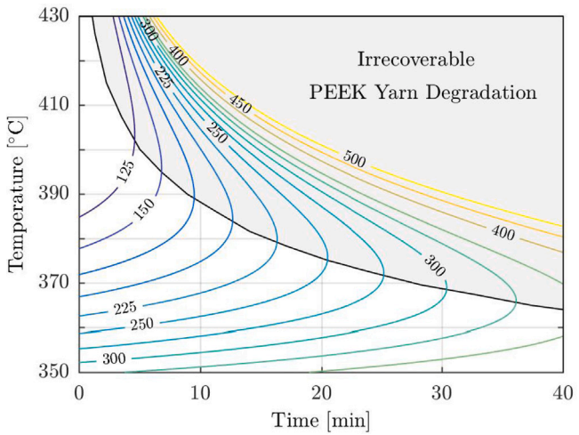
Fig. 7. Iso-viscosity contours computed with the viscosity model accounting for degradation (Eq. (6)) using material parameters identified from viscosity measurements on PEEK yarns (Table 2). The black curve connecting the maximum time of each iso-viscosity level defines a limit of irrecoverable degradation.
