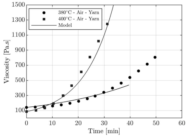
Fig. 3. Comparison of experimental PEEK yarns viscosity (from NCF preform) with the rheological model taking into account the degradation behavior of PEEK yarns (Eq. (6)).
