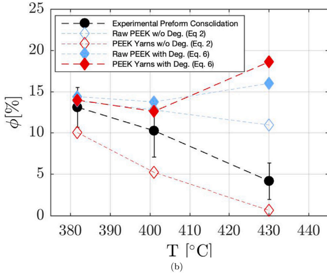
Fig. 10. Comparison of the experimental void contents resulting from processing conditions of (a) 10 min and 25 bar and (b) 20 min and 50 bar ( \bullet ) with the predictions obtained with the viscosity model when considering only the temperature dependence (Eq. (2) without degradation, \diamond ) and when taking into account degradation in addition (Eq. (6), \blacklozenge ). The blue symbols ( \diamond ) correspond to the simulation performed with the parameters identified for the pure matrix, the red symbols ( \diamond ) for the PEEK yarns from the preform. Dotted lines are shown to indicate trends.
