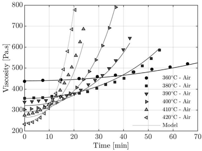
Fig. 2. Comparison of experimental raw PEEK viscosity with the rheological model taking into account the degradation behavior (Eq. (6)).
