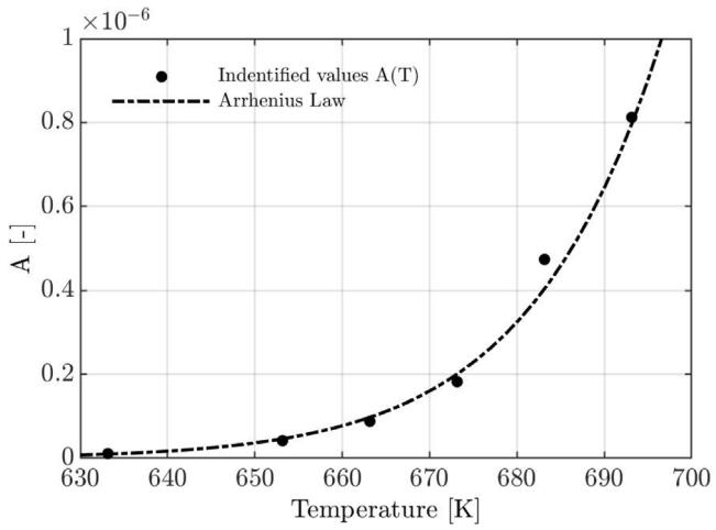
Fig. 6. Kinetic factor A(T) of the viscosity model (Eq. (6)) as a function of temperature for B = 2 and comparison with the prediction given by the Arrhenius law of Eq. (5).
