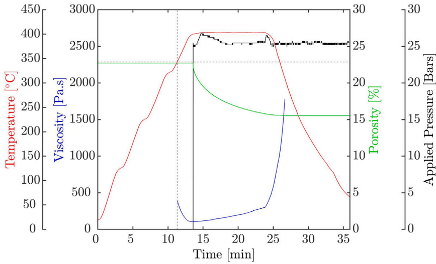
Fig. 1. Processing cycle recorded during the compression molding of 4 plies of CF/PEEK commingled NCF at 400 °C during 10 min under a pressure of 25 bar. The viscosity and porosity are simulated data determined with a rheological model taking into account the degradation behavior of PEEK matrix (Eq. (6)).
