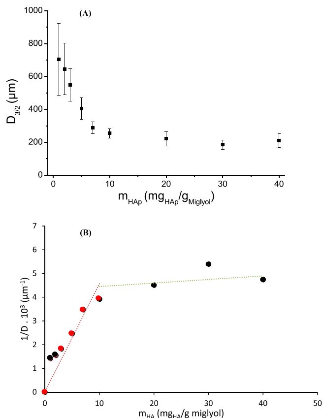
Fig. 6. A) Evolution of the mean Sauter diameter ( D_{3/2} ) of the oil droplets as a function of HA content from 1 to 40 mg HAp /g Miglyol (o/w=75/25–0.5 M NaCl). The error bars represent the standard deviation; B) Evolution of the reverse D_{3/2} of the oil droplets in function of HA content from 1 to 40 mg HAp /g Miglyol (o/w=75/25–0.5 M NaCl). The red points (linear zone of the limited coalescence) are selected to calculate the slope. (For interpretation of the references to colour in this figure legend, the reader is referred to the web version of this article.)
