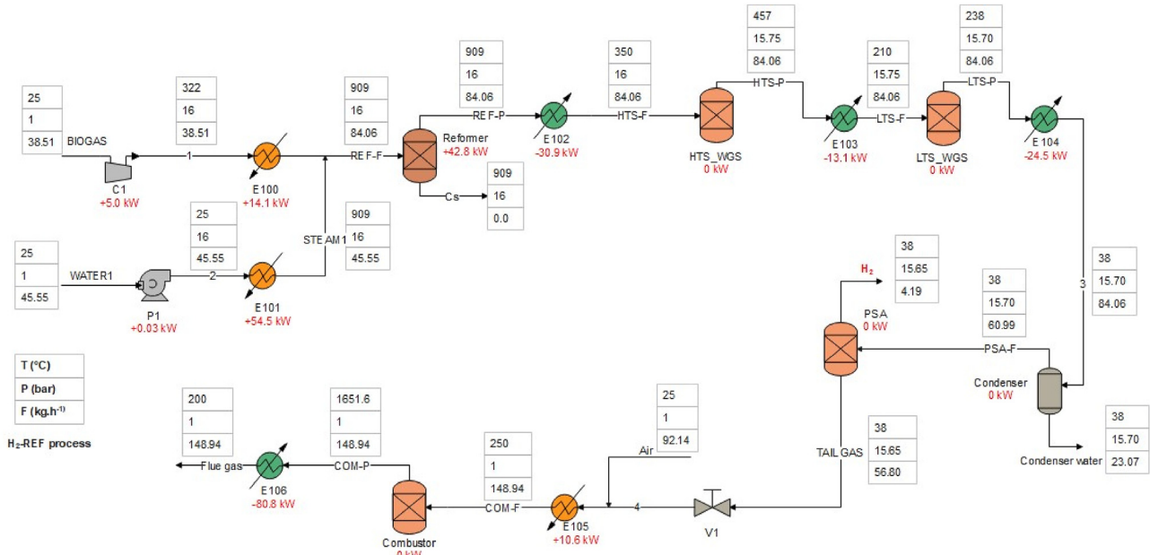
Fig. 1 – Flowsheet of the global hydrogen production process dimensioned by our industrial partner of the VABHYOGAZ3 project with a capacity of 100 kg of H 2 day -1 .
