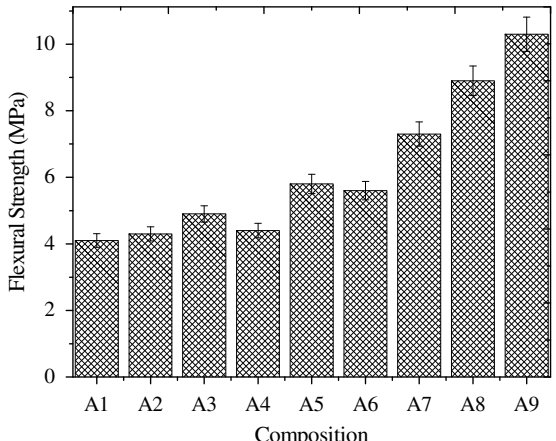
Fig. 8. Flexural strengths of laterite composites.
