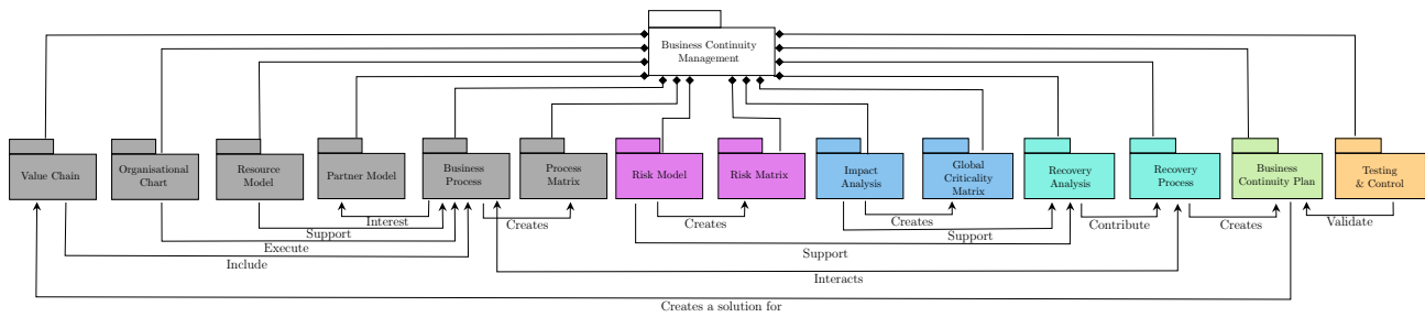
Fig. 2. The overall meta-model of the modeling method for BCM.
