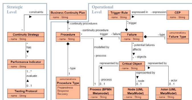
Fig. 1. Meta-model of a business continuity plan (Rejeb, 2013)
