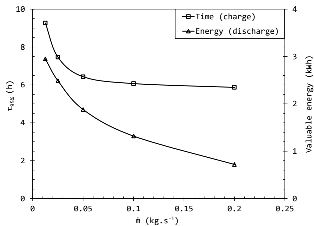
Figure 10. Charging time \tau_{95\%} (left axis) and valuable discharged energy above 45 °C (right axis) as function of the mass flow rate between 43 °C and 70 °C.
