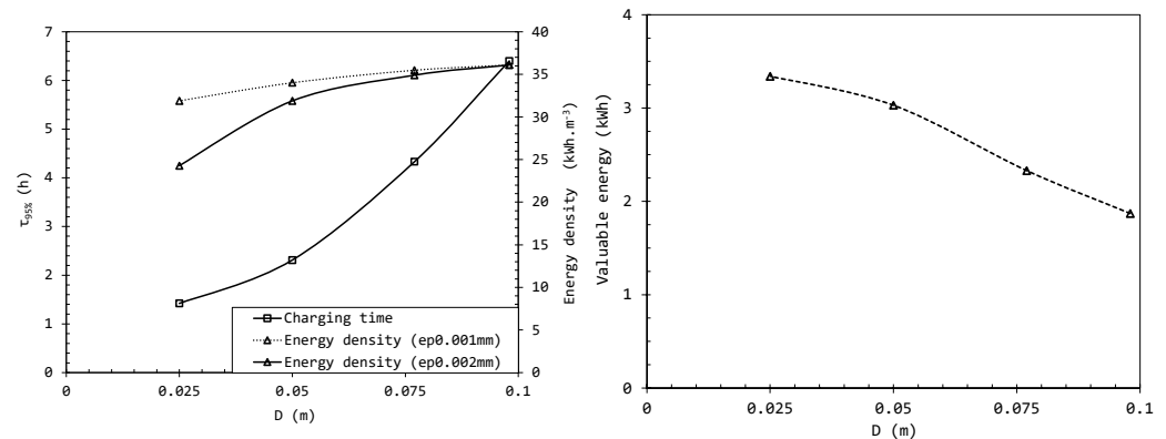
Figure 13. Influence of the nodules' diameters on the charging time \tau_{95\%} (left) and valuable discharge energy above 45 °C (right).
