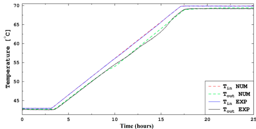
Figure 7. Charge mode from 43 to 69.9 °C at 2 °C/h and 180 L/h.
