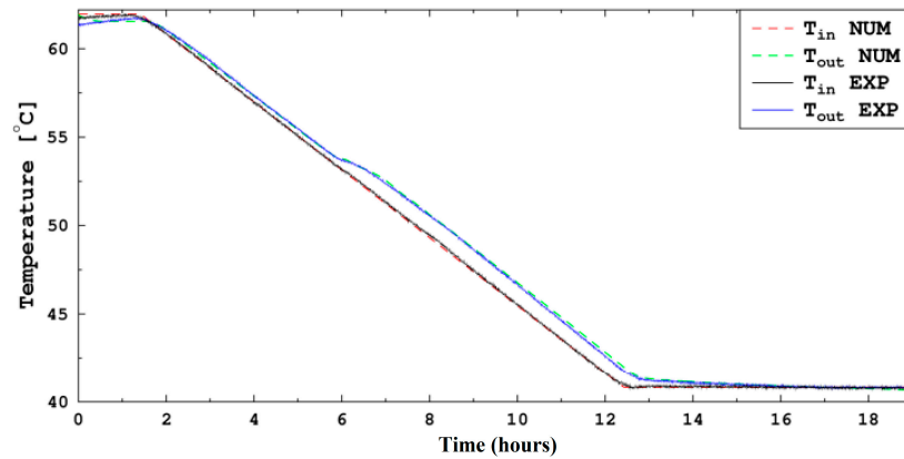
Figure 8. Discharge mode from 62.1 to 40.8 °C at 2 °C/h and 194 L/h.
