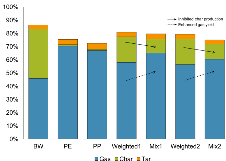
Figure 1. Carbon distribution to pyrolysis products for individual materials and their mixtures.
