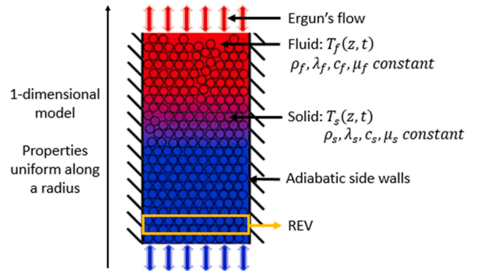
Fig. 3. Thermocline tank model [24]
