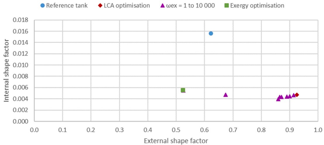
Fig. 14. Shape factors of exergy/LCA optimisations with different weights
