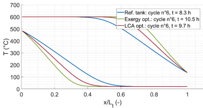
Fig. 8. Evolution of temperature limit profiles depending on the three studied tanks
