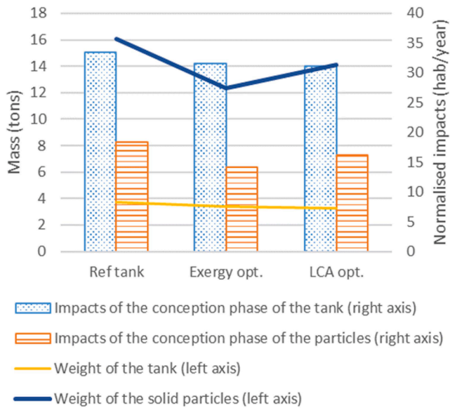
Fig. 10. Environmental impacts of the conception phases (tank and TESM) for the ADP indicator
