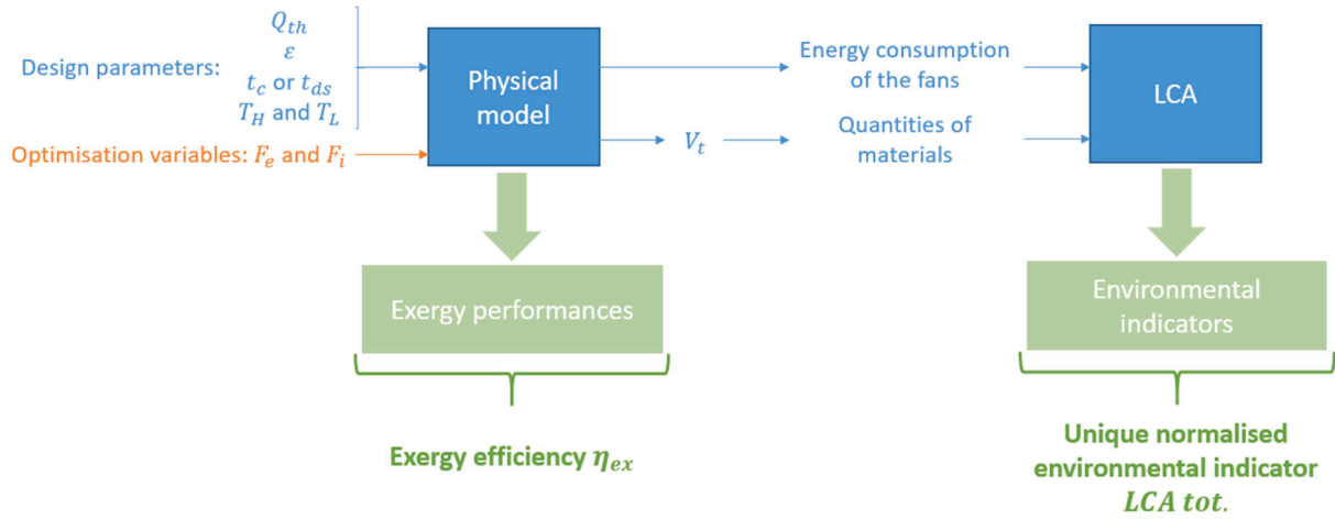
Fig. 5. Overall structure of the multi-criteria optimisation with the inputs and outputs of each model
