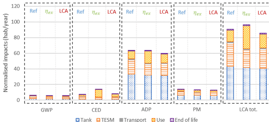
Fig. 9. Comparison of LCA normalised indicators for the different configurations by phases of the life cycle
