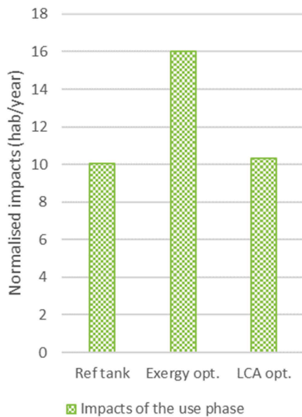
Fig. 11. Environmental impacts of the use phase for the ADP indicator
