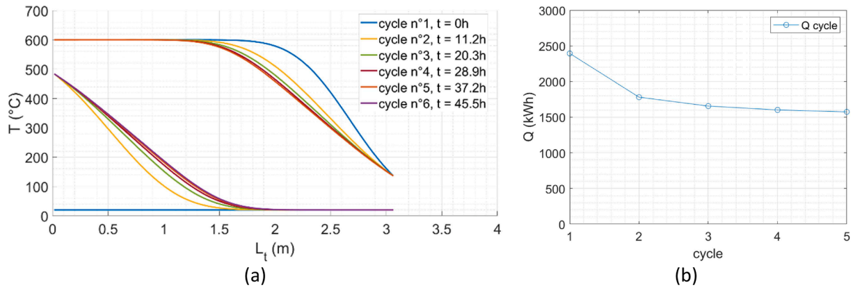
Fig. 7. Temperature limit profiles (a), Internal energy of the tank (b) for Eco-Stock® tank
