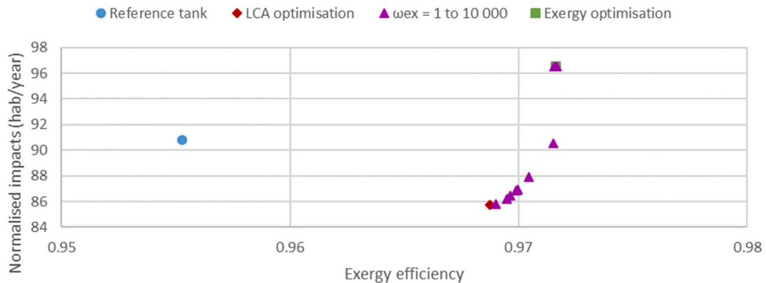
Fig. 13. Pareto graph of exergy/LCA optimisations with different weights
