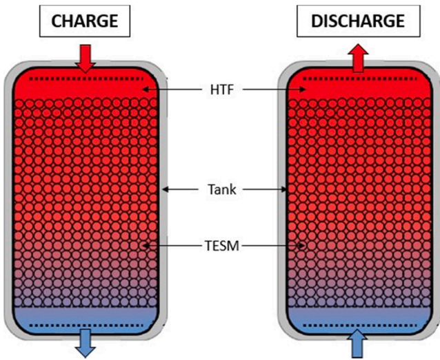
Fig. 1. Thermocline tank working principle
