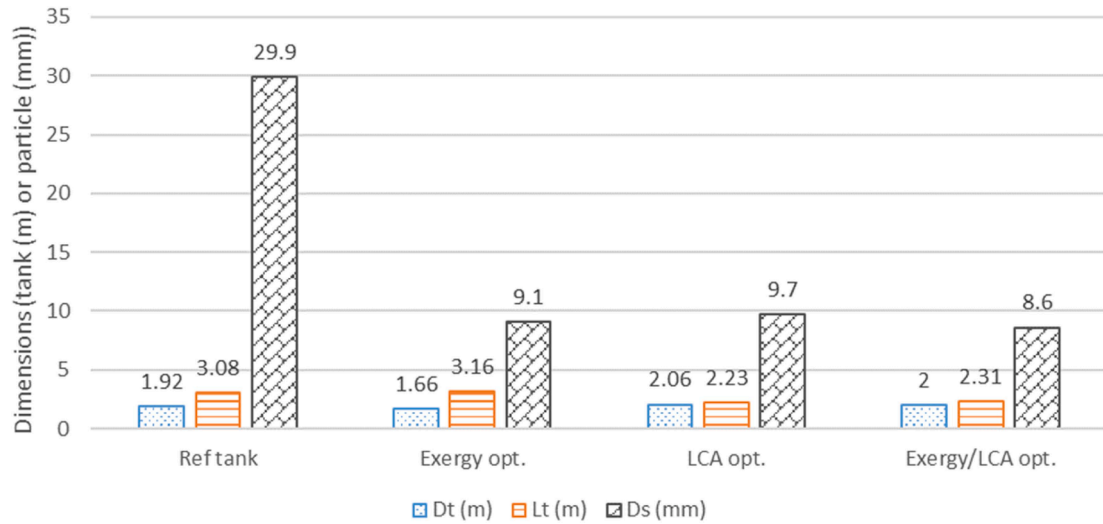
Fig. 15. Comparison between the three different designs: the reference (left), the exergy (middle) and the LCA (right) optimisations
