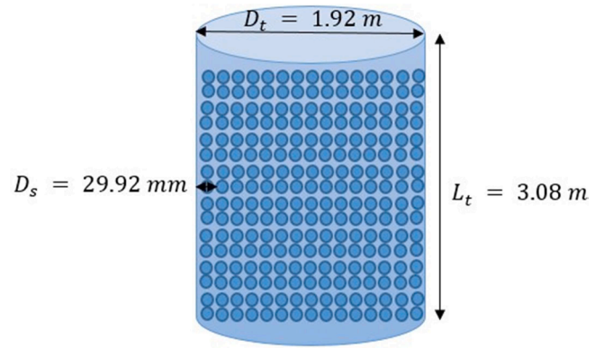
Fig. 6. Dimensions of the Eco-Stock® thermal storage system
