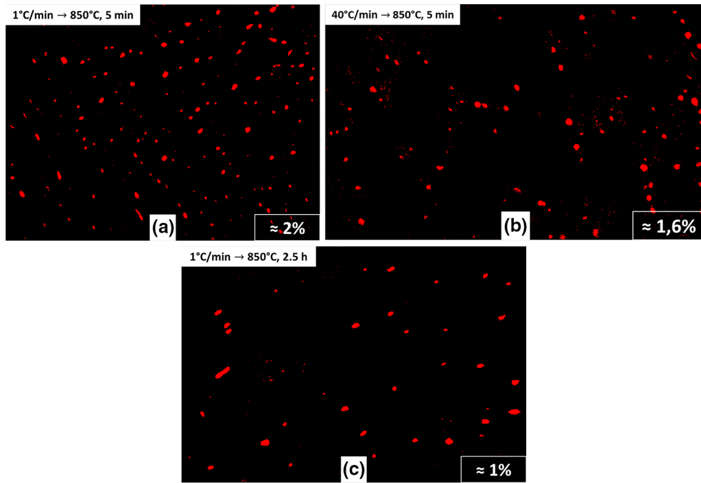
Fig. 10—Image analysis based on the STEM-EDX maps presented in Figs. 8(a) through (c). The \beta -NiAl precipitates from the thresholding process appear in red and the surface fractions estimated are indicated at the bottom right of each image (Color figure online).
