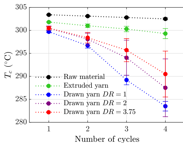
Fig. 4. Temperature of crystallization ( T_c ) against the number of cycles at 400 °C during 20 min, under neutral atmosphere, for all samples. Error bars are representing standard deviations.
