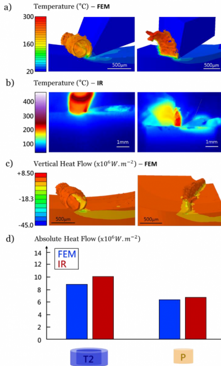
Fig. 5. Experimental (IR) and Numerical (FEM) thermal results – Tube T2 (left), Pin P (right).
