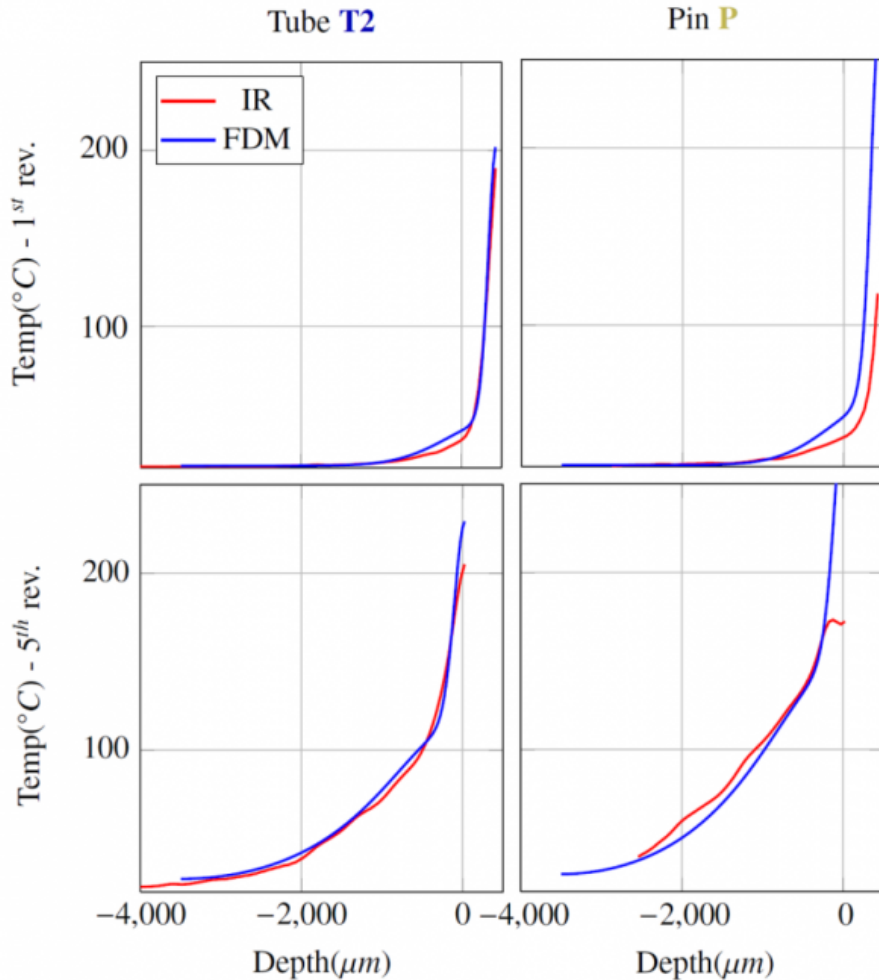
Fig. 6. 2D FDM Model – Temperature profile over 1 revolution (top) and 5 revolutions (bottom) – Tube T2 (left), Pin P (right)
