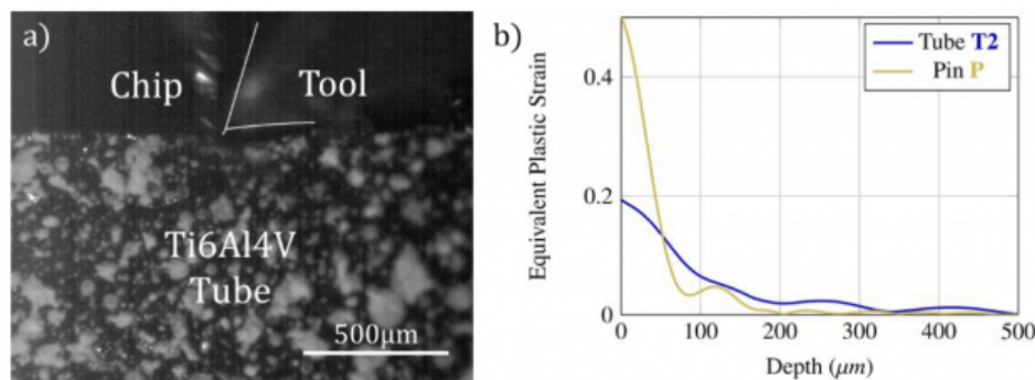
Fig. 4. Visible image and Experimental (DIC) strain results.
