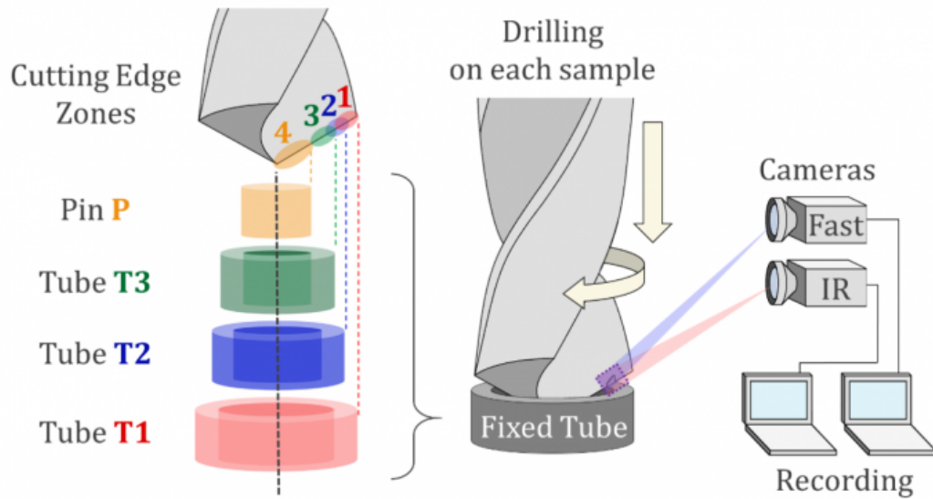
Fig. 1. Experimental set-up
