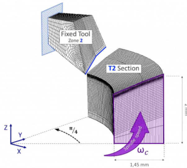
Fig. 2. 3D Thermomechanical Finite Element Model – Tube T2
