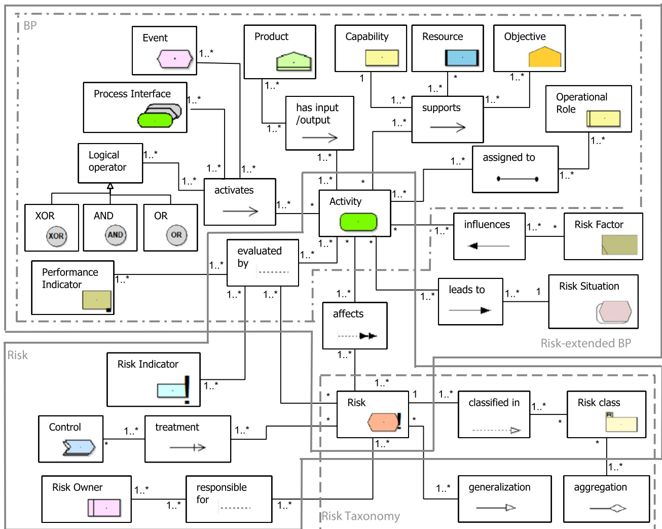
Fig. 9 Excerpt of the implemented e-BPRIM modeling language (syntax and notation)
