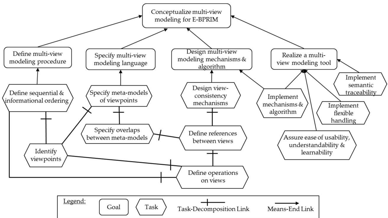
Fig. 4 e-BPRIM multi-view modeling requirements as simplified i* Strategic Dependency model
