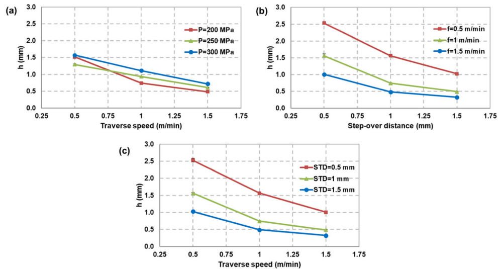
Fig. 14 Effect of the (a) pressure, (b) traverse speed, and (c) step-over distance, on pocket depth
