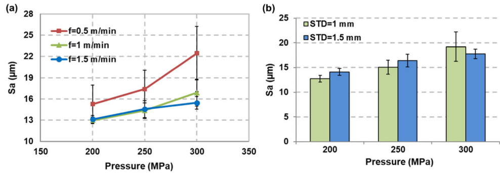
Fig. 4 Effect of the pressure on surface roughness at (a) different traverse speed and (b) different step-over distance
