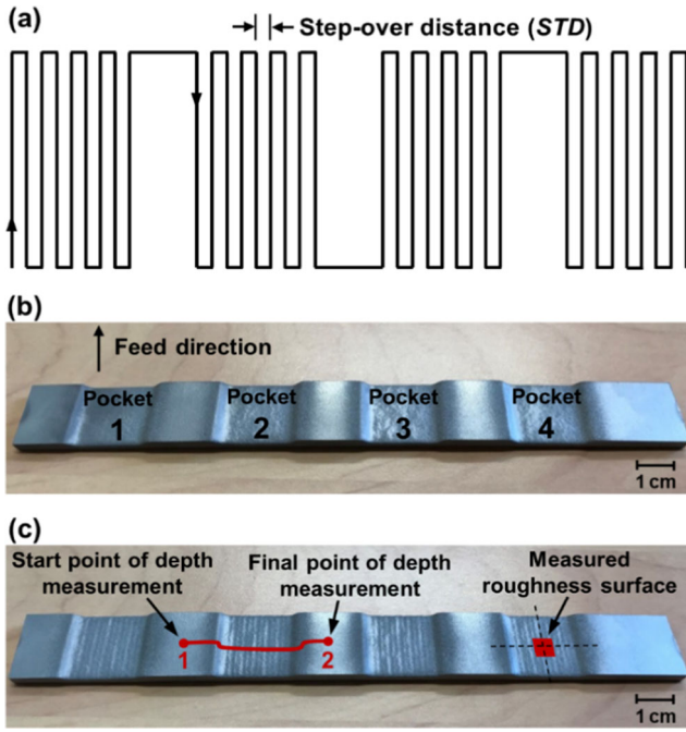
Fig. 2 (a) Tool path; (b) sample machined at P=250 MPa, f=1 m/min, and STD=0.5 mm; (c) location of pocket depth and roughness measurements of the pocket 2 and the pocket 4, respectively, of the specimen milled at P=300 MPa, f=0.5 m/min and STD=1.5 mm
