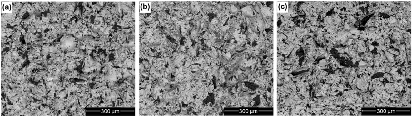
Fig. 10 Micrographs from SEM in \times 150 magnification of surfaces machined at f=1.5 m/min, STD=1 mm and P of (a) 200 MPa; (b) 250 MPa; and (c) 300 MPa
