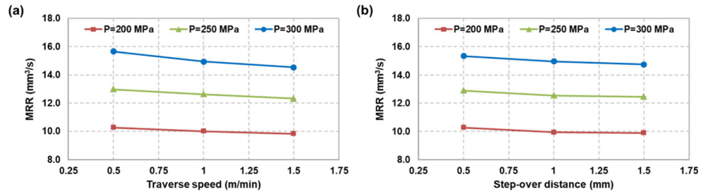
Fig. 15 Effect of (a) the pressure and the traverse speed on the MRR and (b) the pressure and the step-over distance on the MRR
