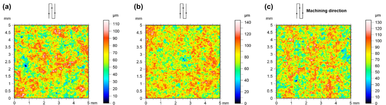
Fig. 9 3D views of the milled surfaces by AWJ of samples machined at 200 MPa of pressure, f=1.5 m/min, P=200 MPa and (a) STD=0.5 mm; (b) STD=1 mm and (c) STD=1.5 mm
