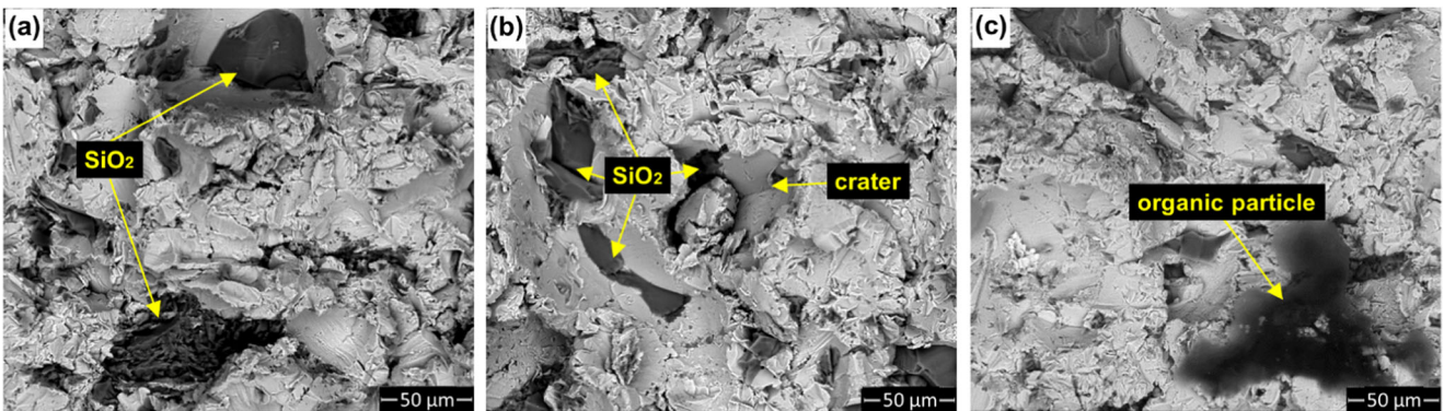
Fig. 13 SEM images of different abrasive particles, (a) silica particles when machining at P = 200 MPa, (b) abrasive particles and crater when machining at P = 250 MPa, and (c) organic particle at when machining at P = 200 MPa
