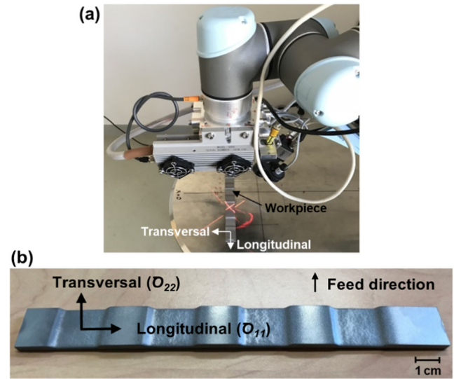
Fig. 3 (a) Setup for the residual stress measurements; (b) residual stress measurement directions
