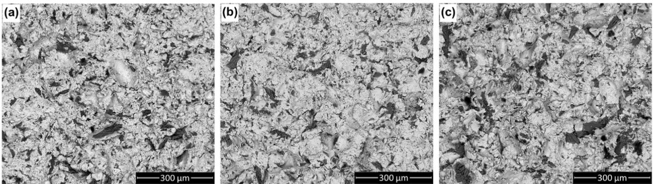
Fig. 11 Micrographs from SEM in \times 150 magnification of surfaces machined at 250 MPa of pressure, STD=1.5 mm and (a) f=0.5 m/min; (b) f=1.0 m/min; and (c) f=1.5 m/min
