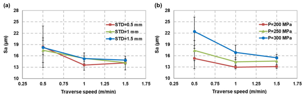
Fig. 5 Mean effect of traverse speed on surface roughness at (a) different step-over distances and (b) at different water pressures
