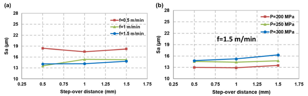
Fig. 6 Effect of step-over distance on surface roughness (a) at different traverse speeds and (b) at different pressures with traverse speed of 1.5 m/min
