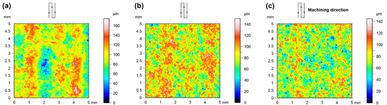
Fig. 8 3D views of the milled surfaces by AWJ of samples machined at 250 MPa of pressure, STD=1.5 mm and (a) f=0.5 m/min; (b) f=1.0 m/min and (c) f=1.5 m/min
