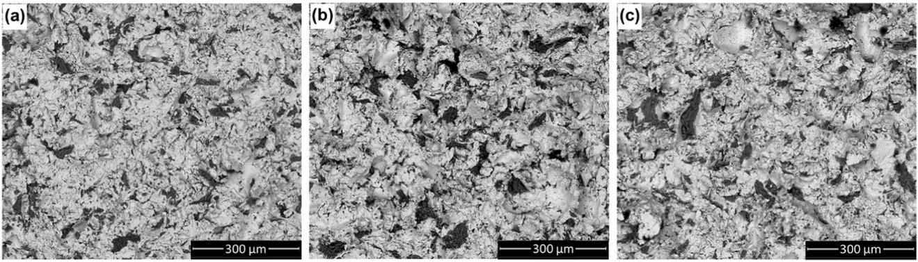
Fig. 12 Micrographs from SEM in \times 150 magnification of surfaces machined at 200 MPa of pressure, f = 1.5 m/min and (a) STD = 0.5 mm; (b) STD = 1 mm; and (c) STD = 1.5 mm
