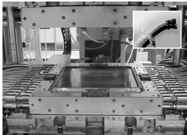
Figure 6 – 3iTech ® induction heated die and copper braided wire inductor
