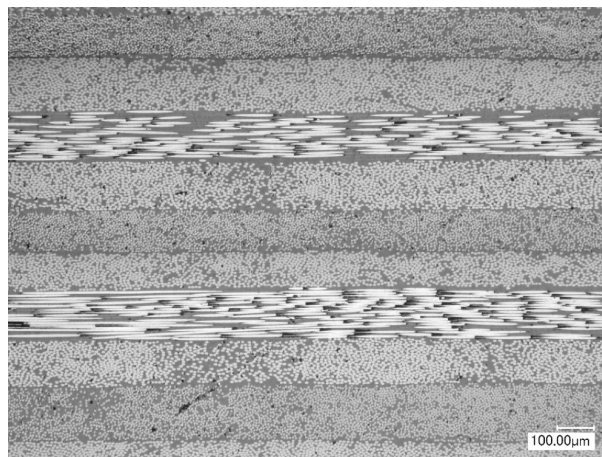
Figure 3 - Microstructure of C/PEEK composite manufactured from prepreg tapes with a conventional hot press
