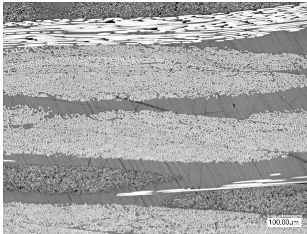
Figure 17 – Microstructure of C/PEEK composite fabricated from powdered prepreg and manufactured with 3iTech ® technology
