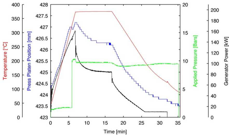
Figure 14 - Processing cycle used for the consolidation of powdered carbon/PEEK prepregs with the Cage System ® technology
