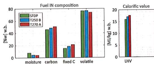
Figure 2: Standard and torrefied pellets after moisture stabilization – average composition and calorific value on w.b.
