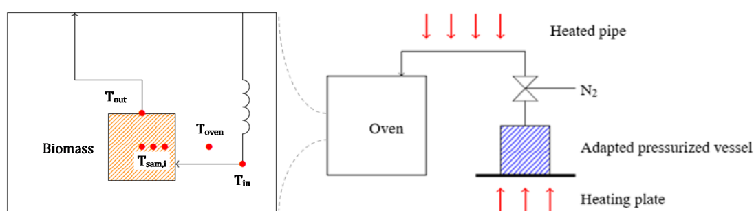
Figure 1. Scheme of the lab-scale facility for torrefaction under moist atmosphere ( H_2O , 100% v/v ) with the detail of the interior of the oven (left).
