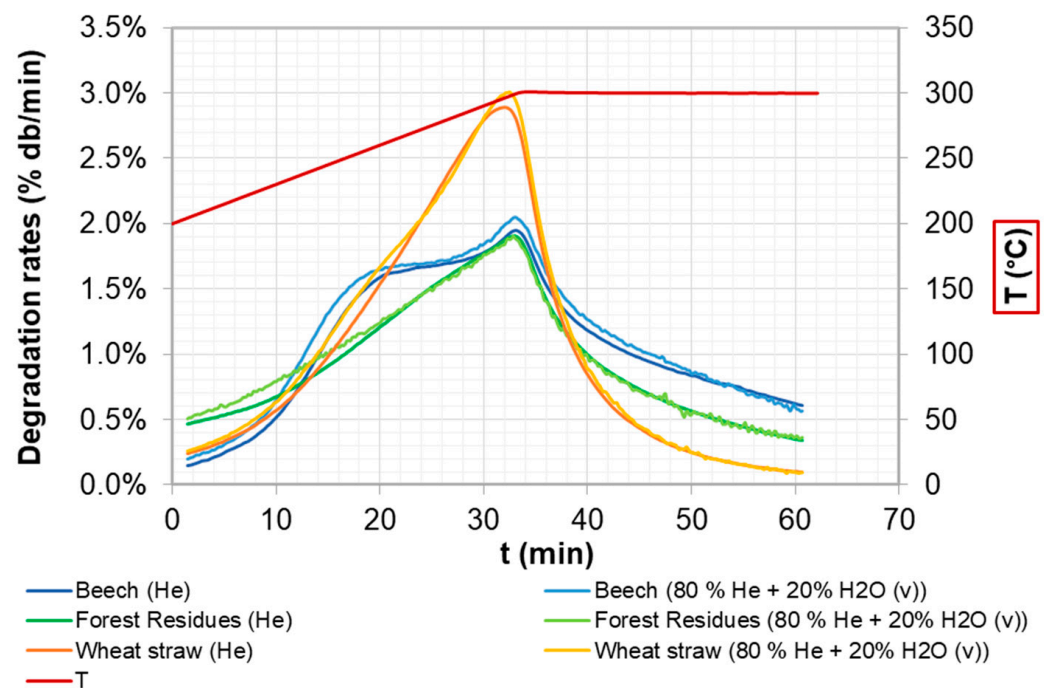
Figure 6. Degradation rate versus time and temperature obtained during torrefaction of beech, forest residues and wheat straw in a TGA under dry (He, 100% v/v) and moist (H 2 O/He, 20% v/v) atmospheres.
