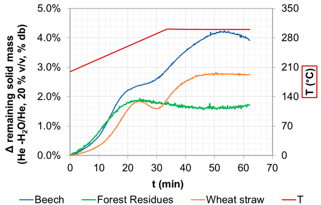
Figure 5. Instantaneous difference in remaining solid mass versus time and temperature from TGA results of the torrefaction of beech, forest residues and wheat straw under dry (He, 100% v/v) and moist (H 2 O/He, 20% v/v) atmospheres.
