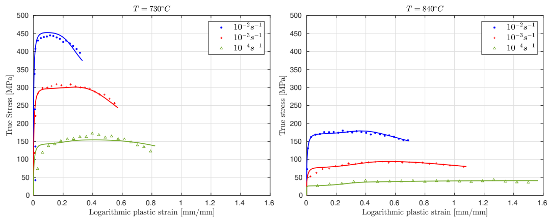
Figure 9. Comparison between experimental and computed stress-strain curves at 730 °C and 840 °C for several strain rate conditions (Model predictions: lines; Experiment: Symbols).
