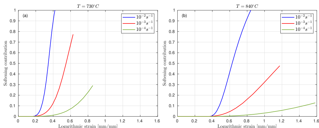
Figure 10. Normalised softening mechanism estimated from variable S at T = 730^\circ\text{C} (a) and T = 840^\circ\text{C} (b).
