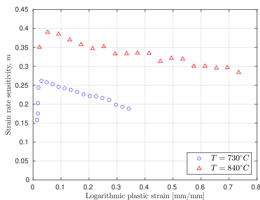
Figure 11. Dependence on the strain rate sensitivity ( m value) on strain at T = 730^{\circ}\text{C} and T = 840^{\circ}\text{C} .
