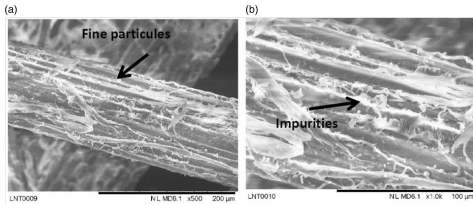
Figure 8. SEM image of untreated Doum palm fiber: (a) Magnificationx 500; (b) Magnificationx1000.
