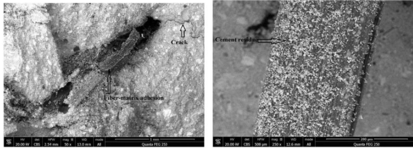
Figure 17. Break surface of cement mortar reinforced with treated fiber.
