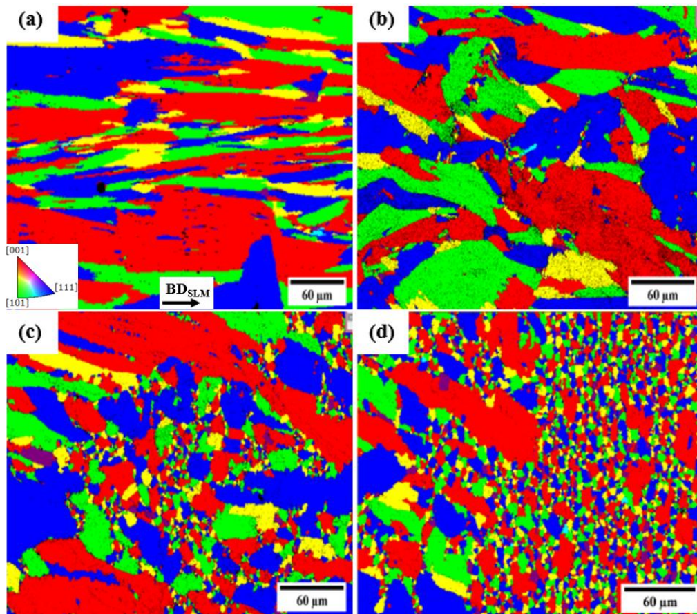
Figure 7. EBSD grain map in the as-SLM IN718 after the LFW to AD730 TM alloy: (a) in the BM zone, (b) in the BM+TMAZ, (c) in the TMAZ, and (d) in the TMAZ+WZ. IPF map and building direction of as-SLM part are shown.
