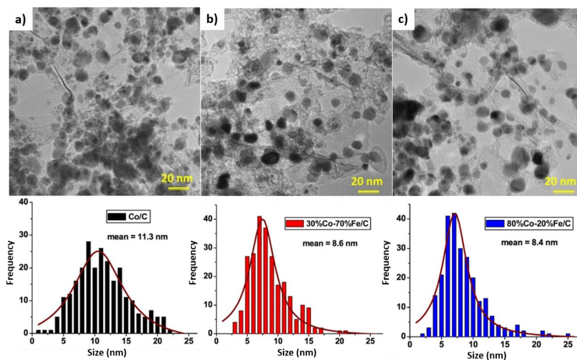
Figure 22. TEM micrographs and particle size distribution of plasma synthesized catalysts. a) Co/C; b) 30%Co-70%Fe/C; and c) 80%Co-20%Fe/C samples. Reprinted with permission from Ref [179]. Copyright 2018 Springer Nature.
