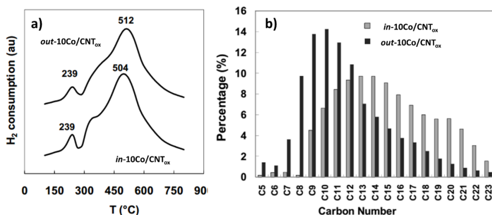
Figure 10. a) \text{H}_2 -TPR profiles for in-10Co/CNT ox and out-10Co/CNT ox catalysts; and b) cold trap product distribution for both the in-10Co/CNT ox and out-10Co/CNT ox catalysts. (T = 220 °C, P = 20 bar and \text{H}_2/\text{CO} = 2 ). Adapted from ref [122].
