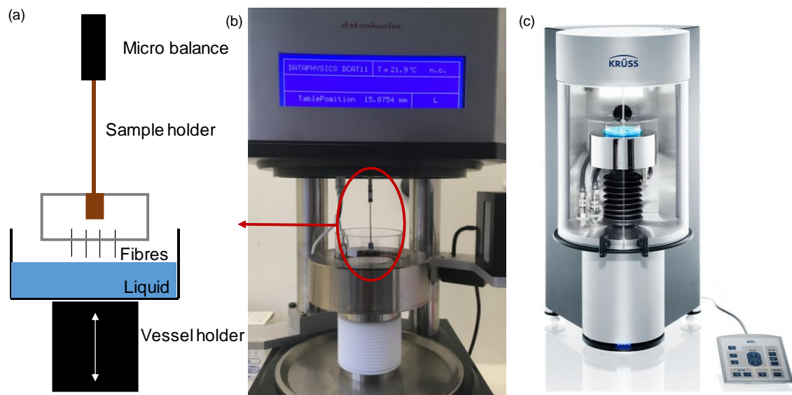
Figure 1. (a) Schematic representation of the vertical mounting of four fibres during testing, (b) DCAT11 tensiometric device and (c) K100SF tensiometric device.
