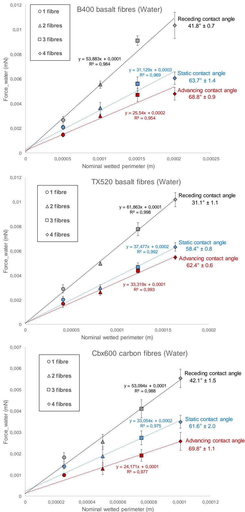
Figure 5. Measurements of contact angles in water for B400 basalt fibres, TX520 basalt fibres and Cbx600 carbon fibres
