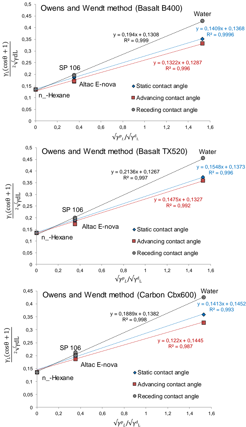
Figure 6. Linear fits for basalt and carbon fibres surface energies as a function of contact angle.
