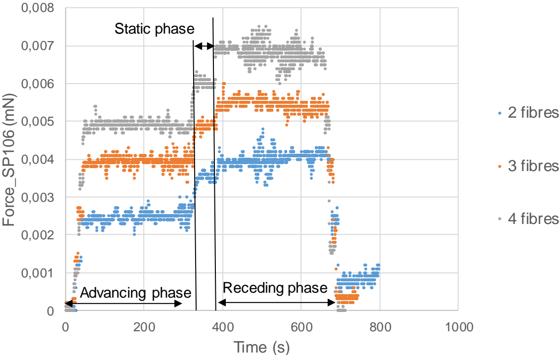
Figure 2. Example of a complete cycle for two, three and four B400 basalt fibres in SP106 resin with the DCAT11 tensiometer.
