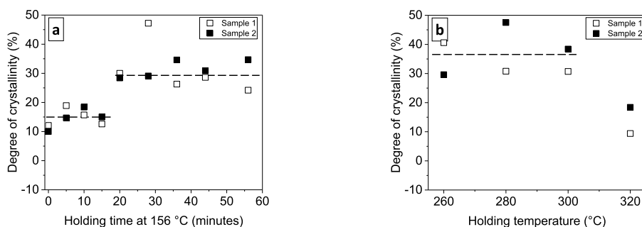
Fig. 6. Degree of crystallinity calculated by DSC for PEEK sample obtained: a) from glassy state; b) from melted state. Each analysis were performed two times. The absolute uncertainty is lower than 0.4% and not represented on the graphic. Dashed lines are guides to the eyes.
