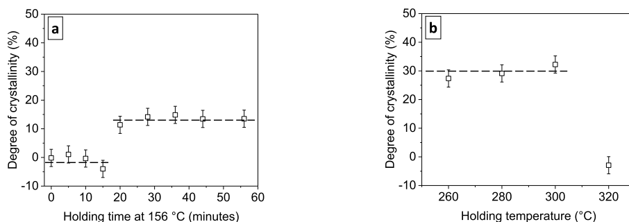
Fig. 4. Degree of crystallinity calculated from density for PEEK samples obtained: a) from glassy state; b) from melted state. The absolute uncertainty is 4%. Dashed lines are guides to the eyes.
