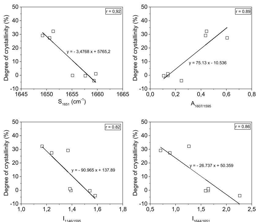
Fig. 12. Value of Raman's indicator according to the degree of crystallinity determined by density; Line: linear regression of the values; r: coefficient of correlation.
