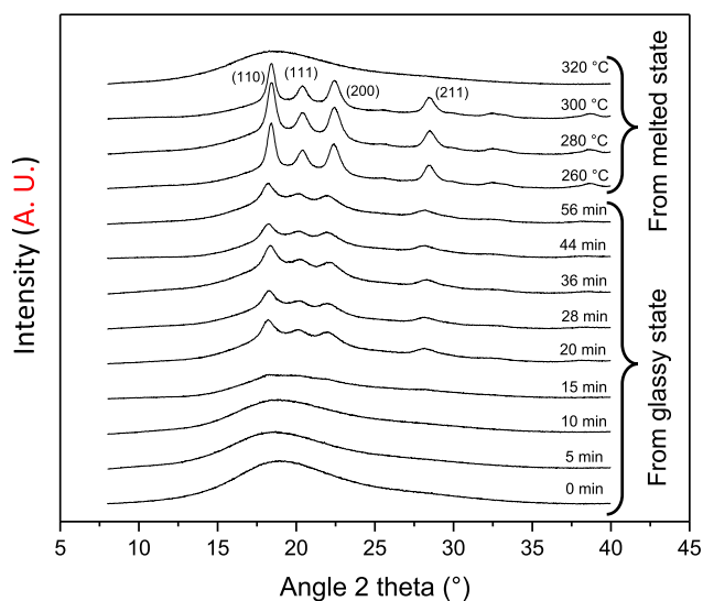
Fig. 7. Diffractogram for PEEK sample obtained from glassy state and from melted state.
