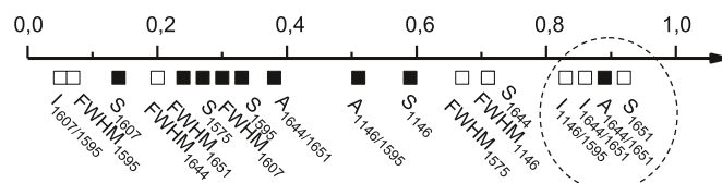
Fig. 10. Absolute values of correlation coefficient of Raman's indicator with the degree of crystallinity determined by density: positive value (■) and negative value (□).
