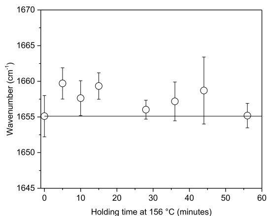
Fig. 11. The band shift \delta_{C-CO-C} for glassy samples. The line indicates the values of the untreated film PEEK. Error bars represented the standard deviation.
