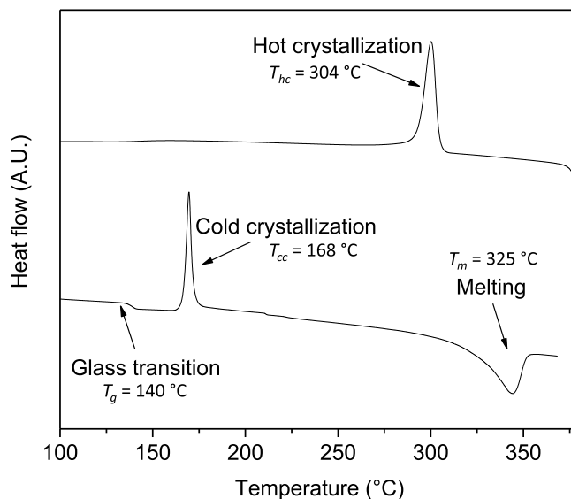
Fig. 5. Thermogram for the untreated sample of PEEK: 1st heating and cooling. crystallinity, two-times higher than for glassy samples.
