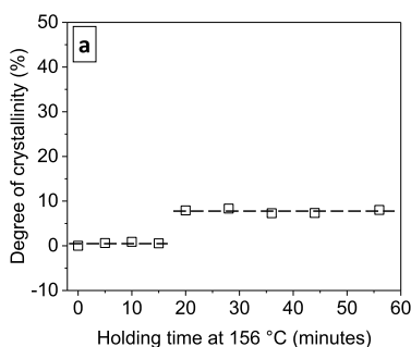
Fig. 8. Degree of crystallinity calculated by XRD for PEEK samples obtained a) from glassy state; b) from melted state. The absolute uncertainty is lower than 0.5% and not represented on the graphic. Dashed lines are guides to the eyes.
