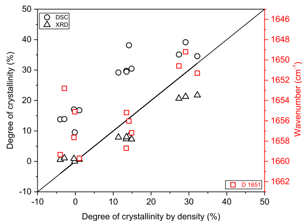
Fig. 13. Degree of crystallinity according to the technique. S_{1651} : wavenumber of the band 1651\text{ cm}^{-1} . The line indicates the ratio conservation. S_{1651} : wavenumber of the band 1651\text{ cm}^{-1} .
