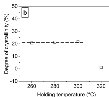
Fig. 8. Degree of crystallinity calculated by XRD for PEEK samples obtained a) from glassy state; b) from melted state. The absolute uncertainty is lower than 0.5% and not represented on the graphic. Dashed lines are guides to the eyes.
