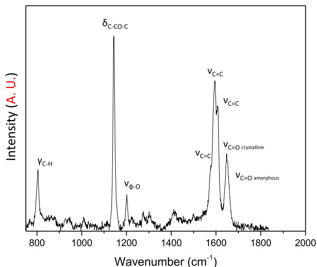
Fig. 9. Spectrum of the PEEK untreated sample. \gamma : out-of-plane bending; \delta : bending or scissoring; \nu : stretching.
