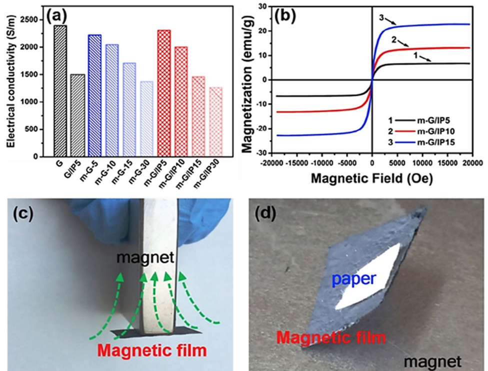
Fig. 10 Conductive and lightweight graphene/iron pentacarbonyl porous films in a Electrical conductivities of graphene and its derivative films; b Hysteresis loops of m-G/IP porous films; c, d Digital images showing the magnetic property of m-G/IP5 porous films [88]
